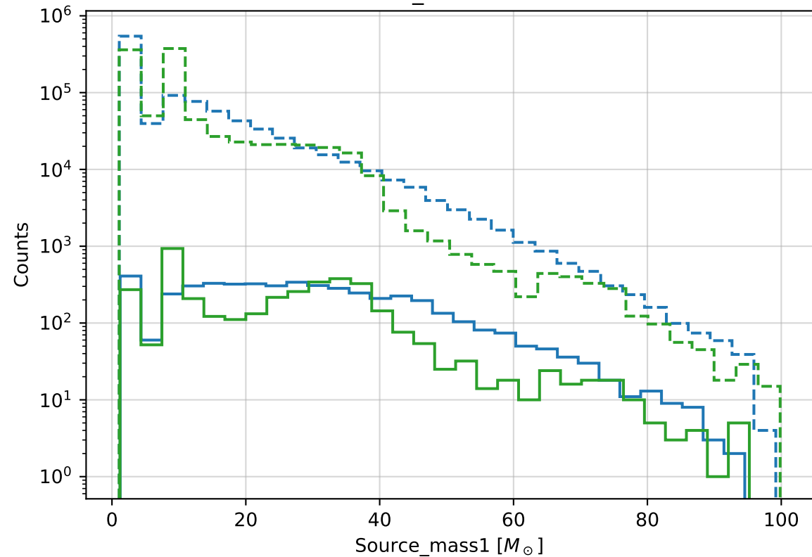
Distribution of Source_mass1: GWTC-3 vs GWTC-4
