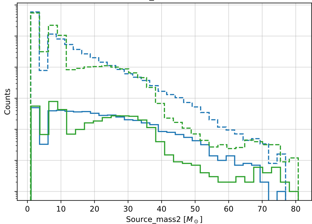
Distribution of Source_mass2: GWTC-3 vs GWTC-4
