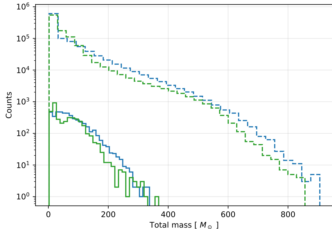
GWTC-3 vs GWTC-4: Total mass
