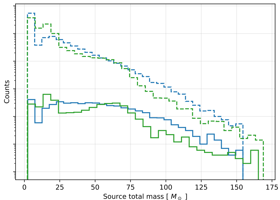
GWTC-3 vs GWTC-4: Source total mass
