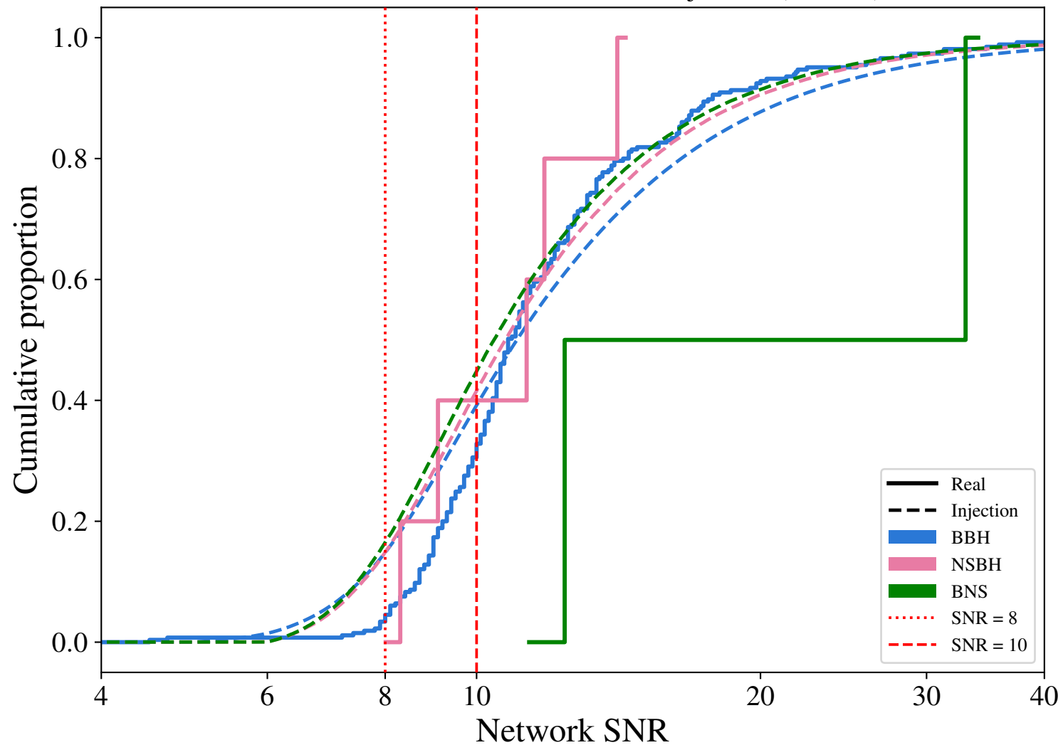
SNR ECDF: real detections vs. found injections (O1-O4b)
