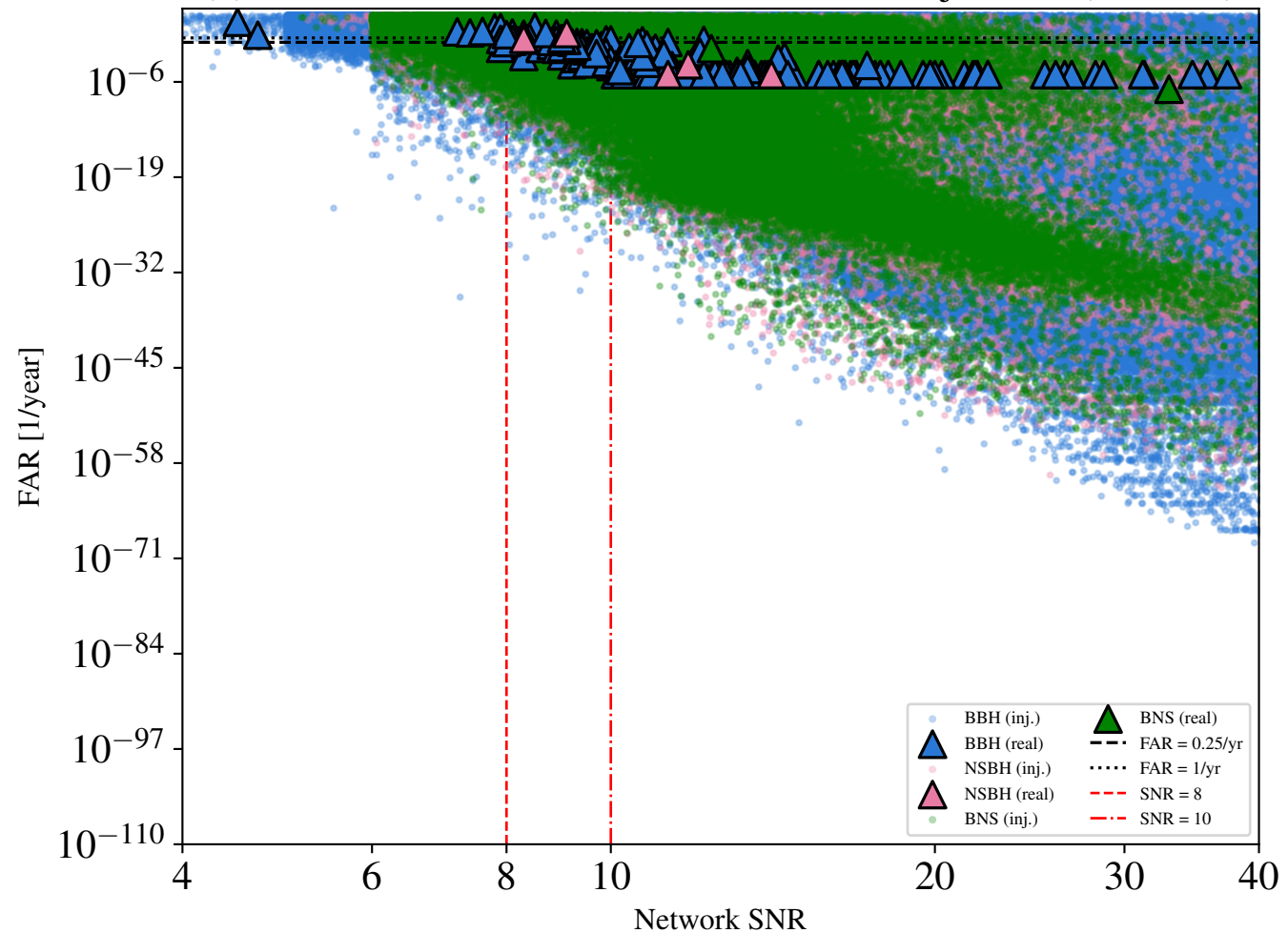
(b) FAR vs. SNR: real detections vs. found injections (O1-O4b)
