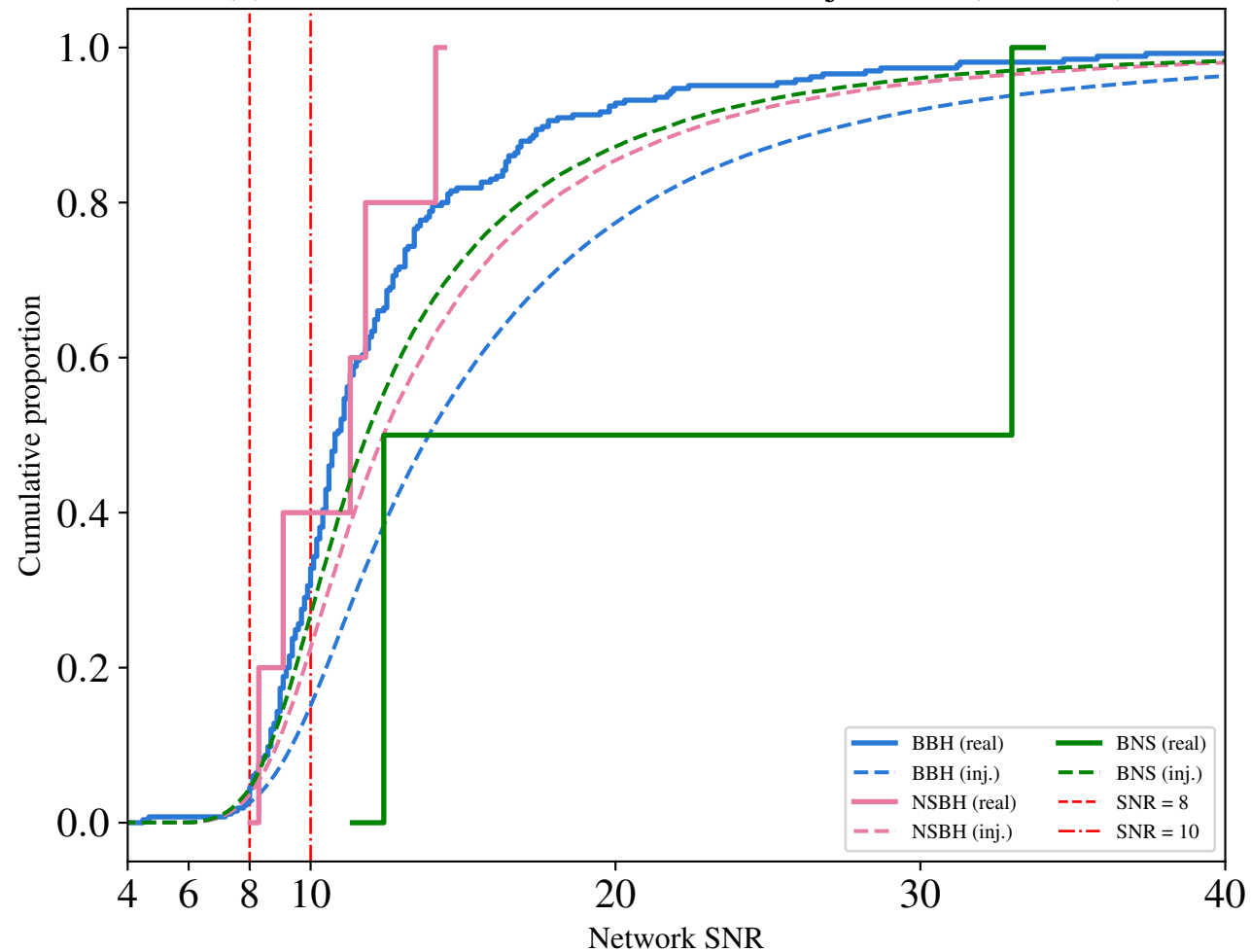
(a) SNR: real detections vs. found injections (O1-O4b)
