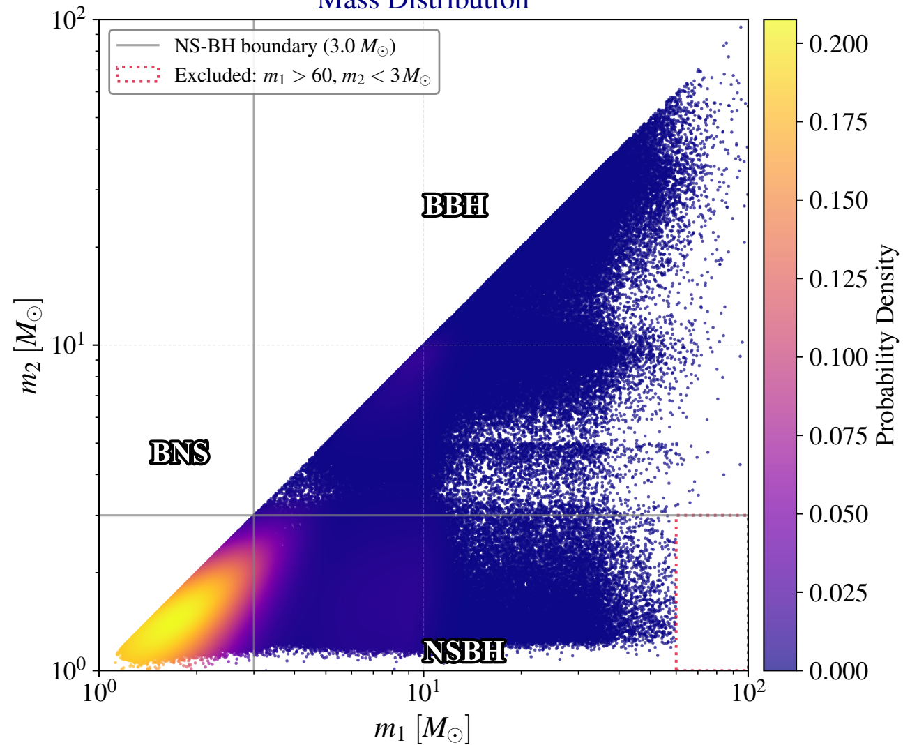
Mass Distribution
