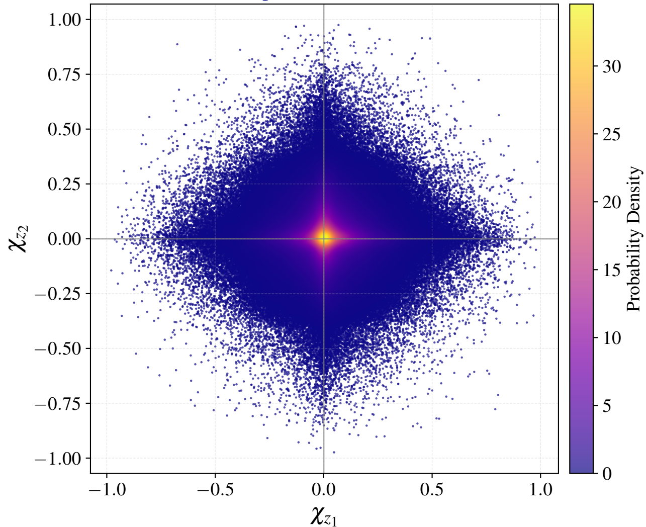
Spin Distribution
