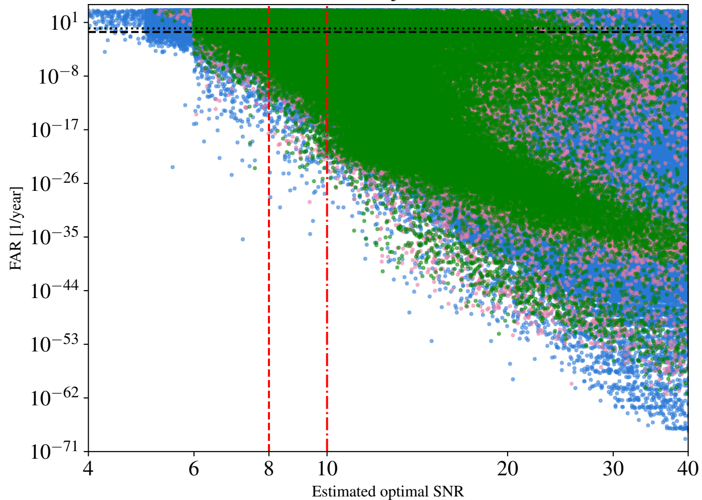
FAR vs SNR, all injections (O1-O4b)
