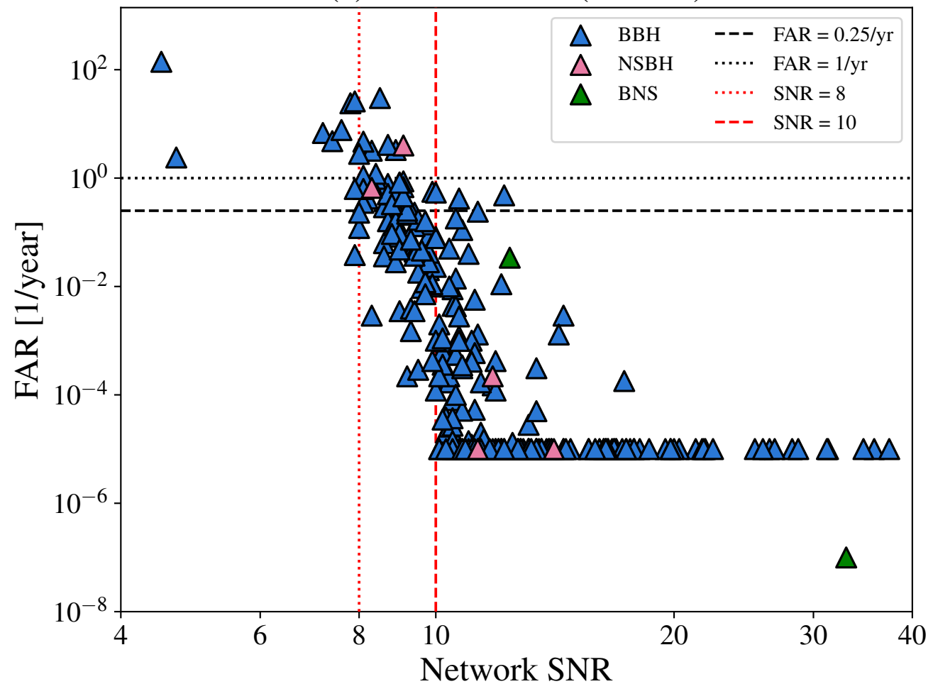
(b) Real detections (O1-O4b)
