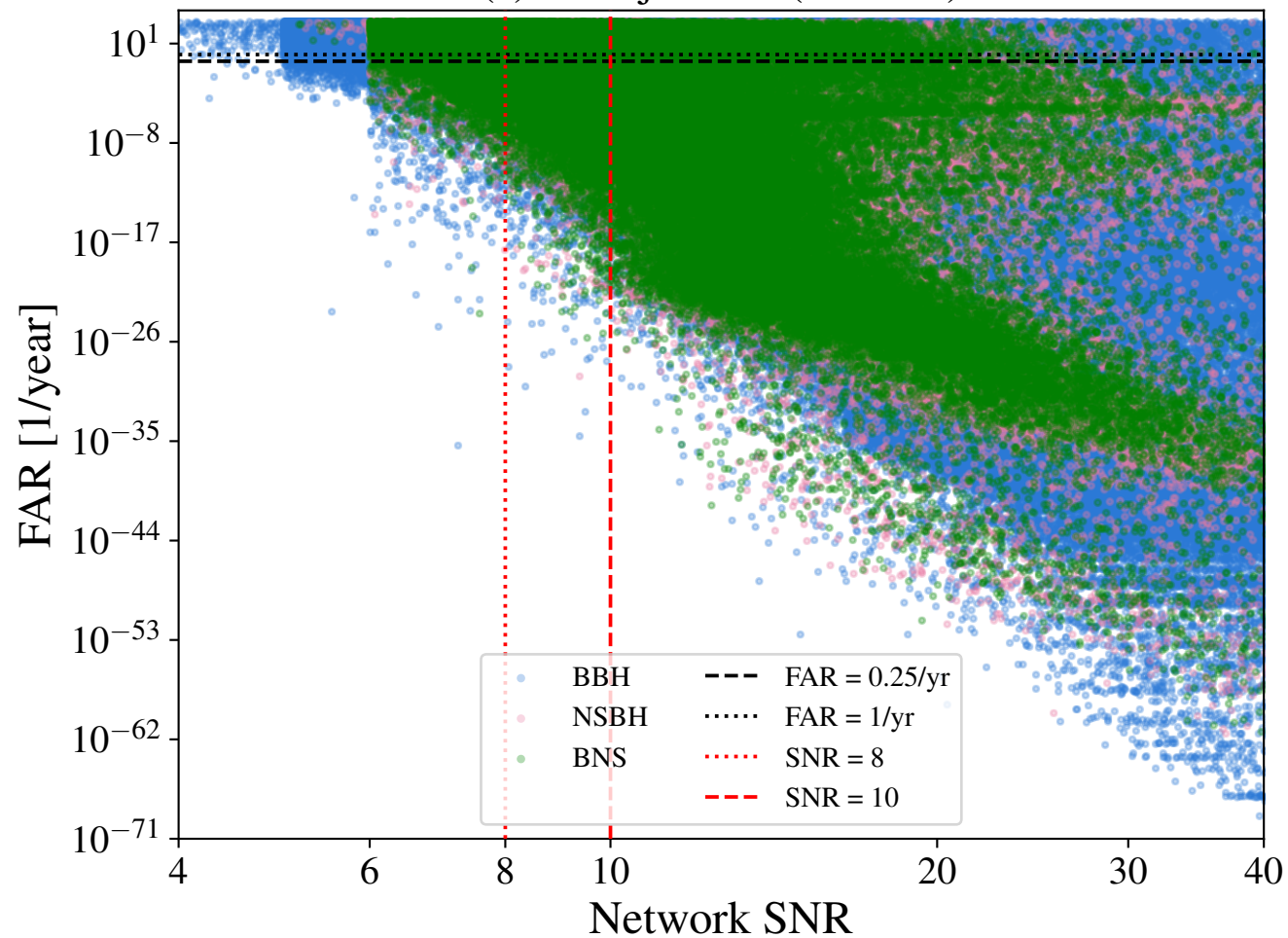
(a) All injections (O1-O4b)
