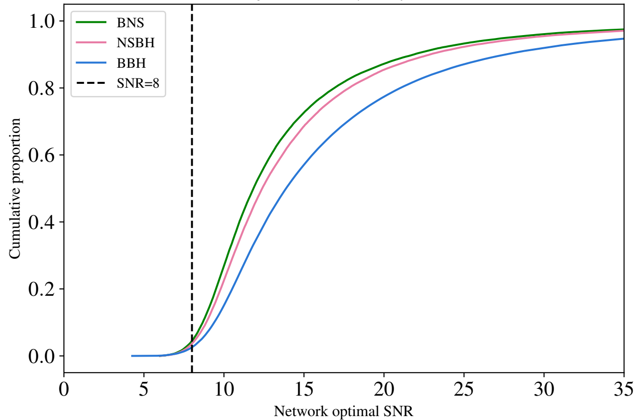
O1-O4b injections (FAR \leq 0.25/yr), cumulative
