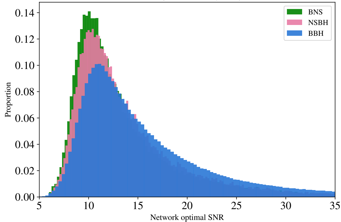
O1-O4b injections (FAR \leq 0.25/yr)
