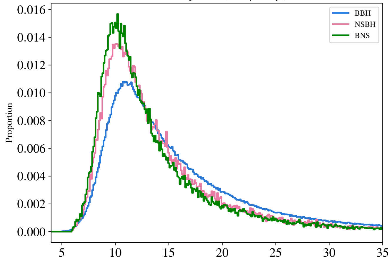
O1-O4b injections (FAR \leq 0.25/yr)
