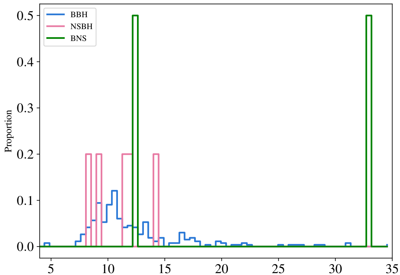
O1-O4b injections (FAR \leq 0.25/yr)
