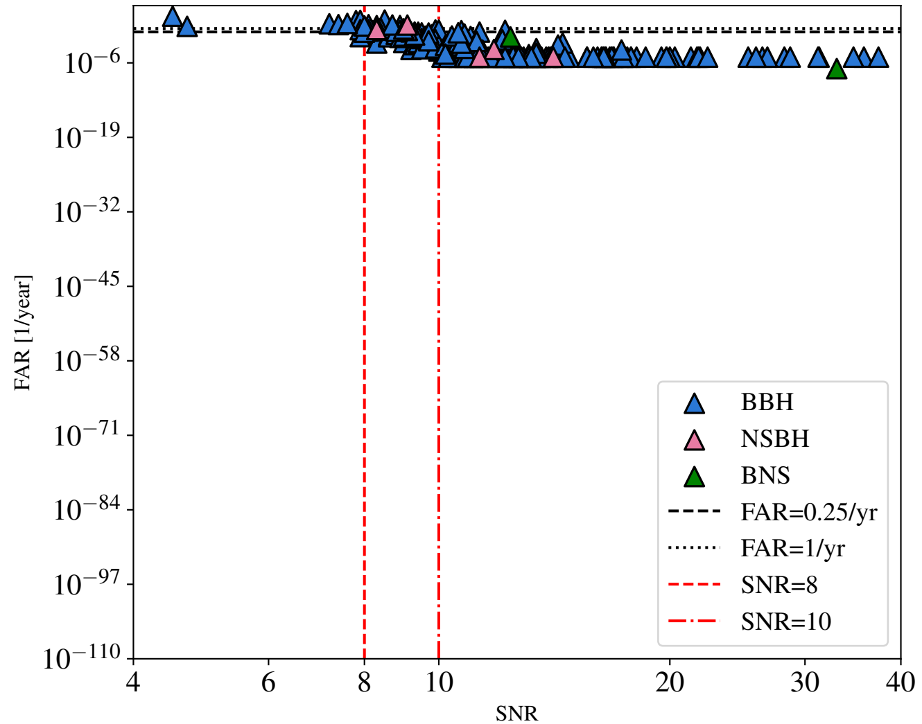
FAR vs SNR, real detections (O1-O4b)
