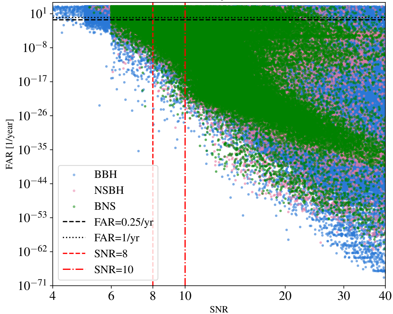
FAR vs SNR, all injections (O1-O4b)
