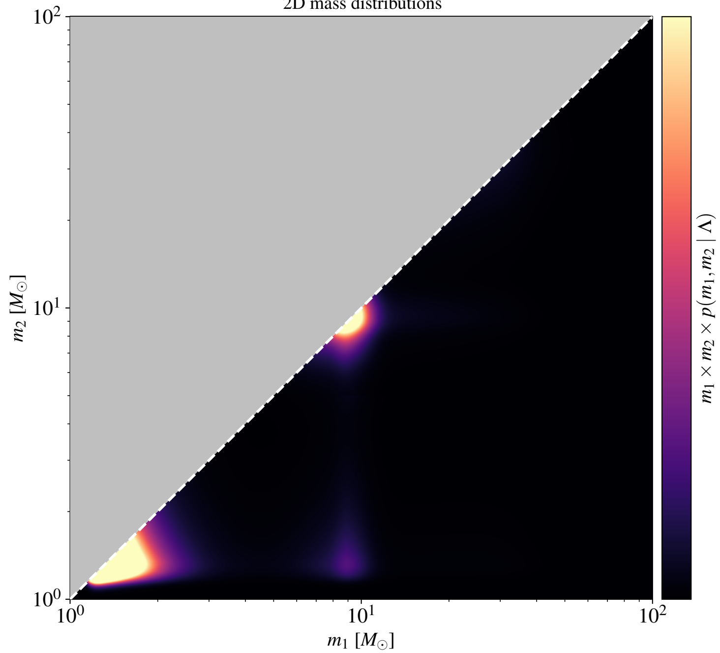
2D mass distributions
