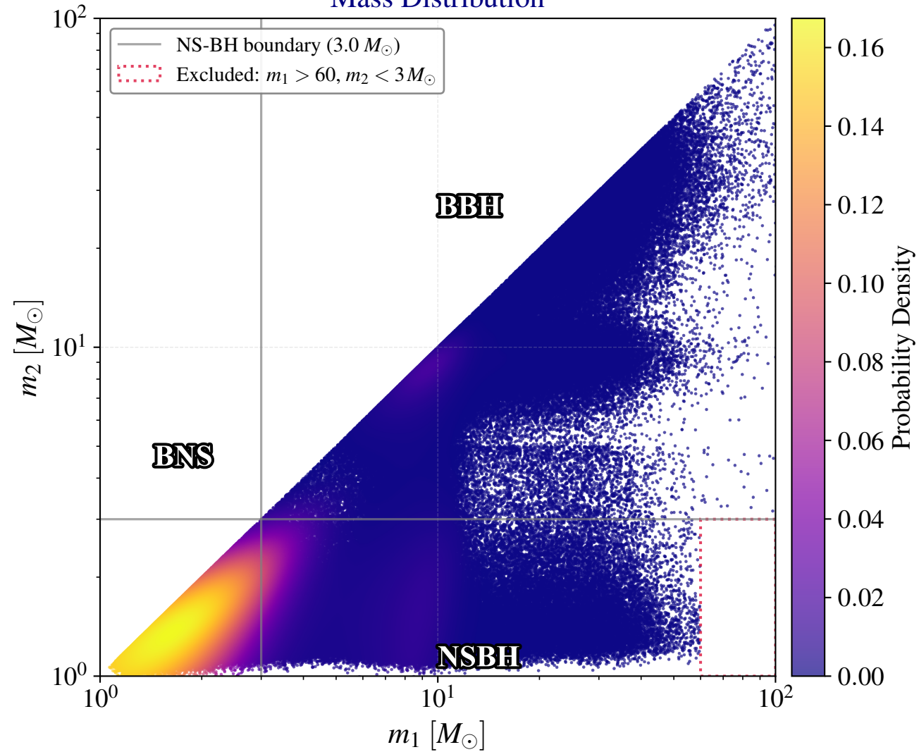
Mass Distribution
