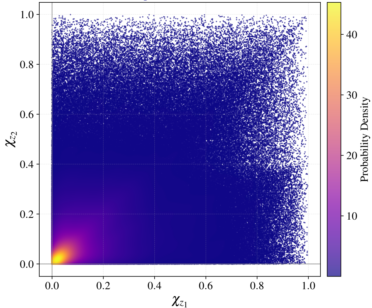
Spin Distribution
