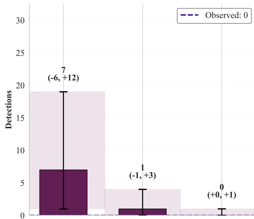
O4a (7.79 months)
