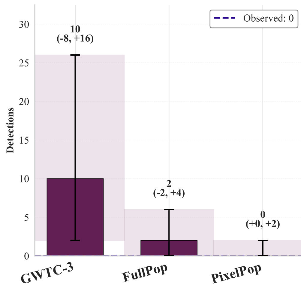
O4b (9.63 months)
