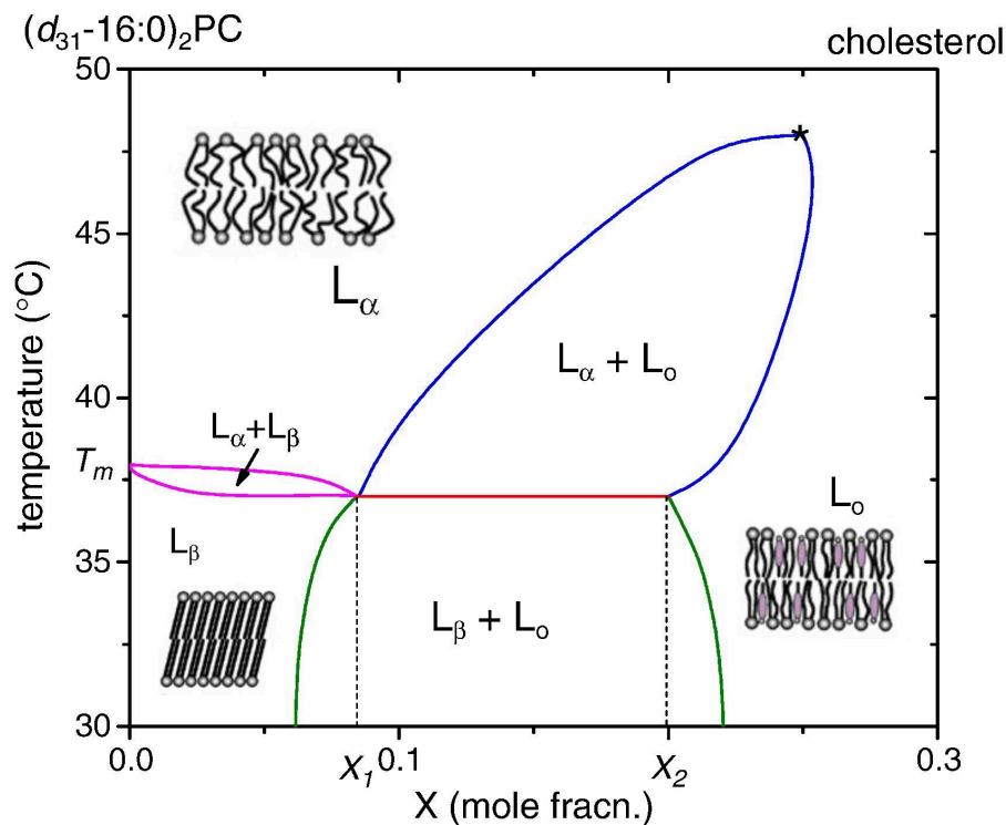
Figure 2 — Phase diagram of DPPC-cholesterol mixture as a function of temperature. Adapted from [12]. © Elsevier (2010), reproduced with permission. 1
