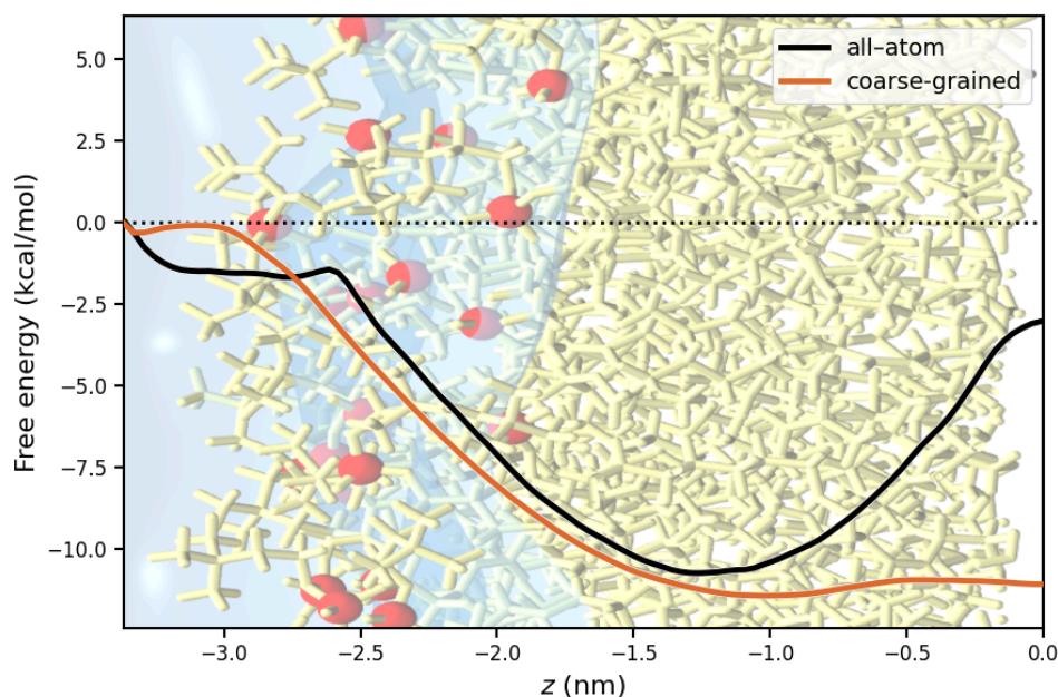
Figure 11 — Potential of mean force associated with CP55,940 insertion into a DOPC bilayer obtained at atomistic and coarse-grained resolutions.
