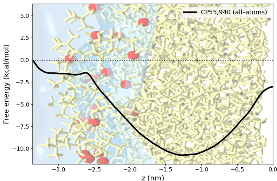
Figure 6 — Potential of mean force computed for a CP55,940 ligand approaching a DOPC membrane in all-atoms. An indicative illustration is set in the background to visualize the leaflet.
