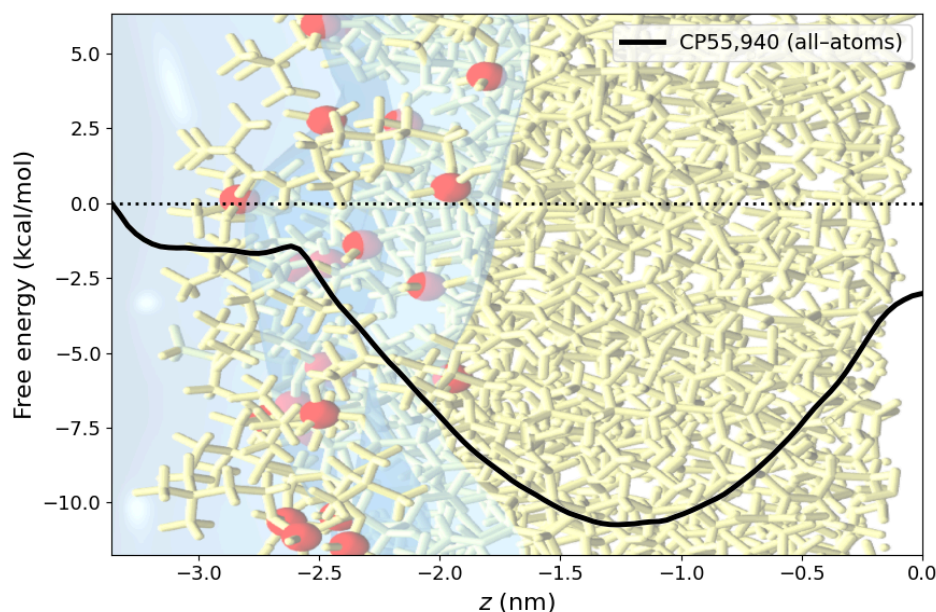
Figure 6 — Potential of mean force computed for a CP55,940 ligand approaching a DOPC membrane in all-atoms. An indicative illustration is set in the background to visualize the leaflet.
