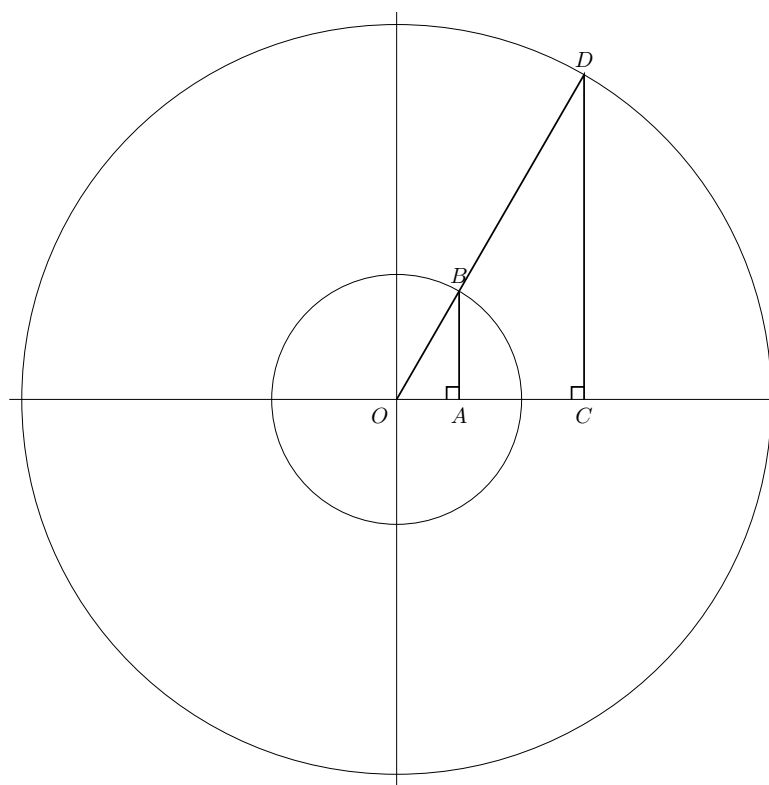
Figure 20 Circles with Similar Triangles
