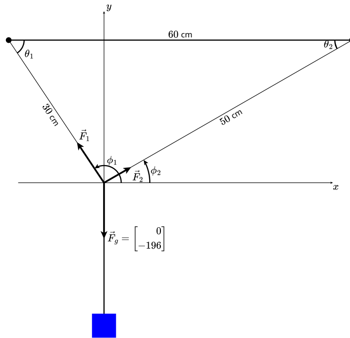
Figure 67 A Weight Suspended Asymmetrically with Axes Imposed
