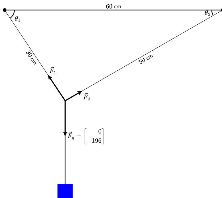
Figure 62 A Weight Suspended Asymmetrically
