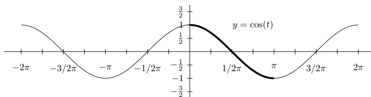
Figure 49 The Cosine Function and its Principle Branch
