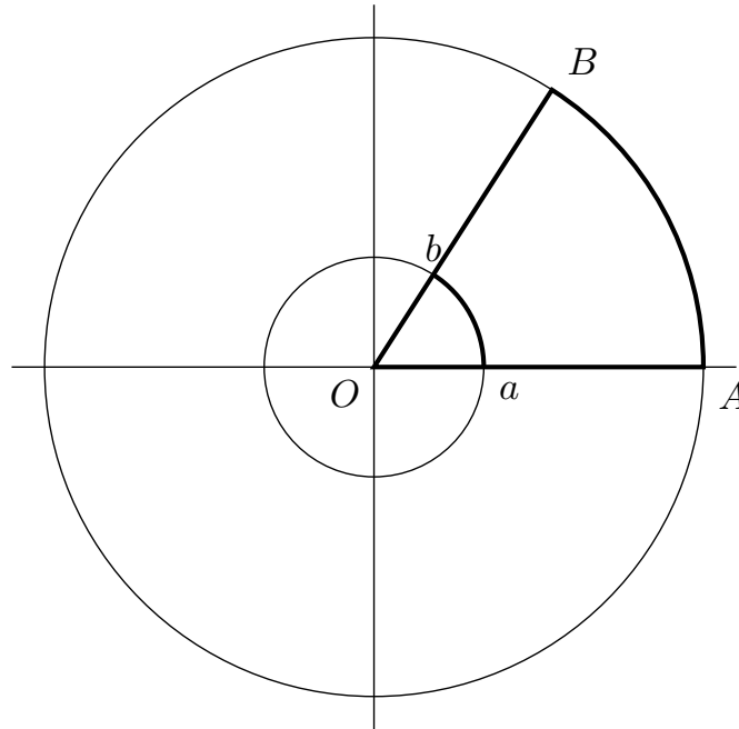
Figure 14 One radius of arc length on two different circles
