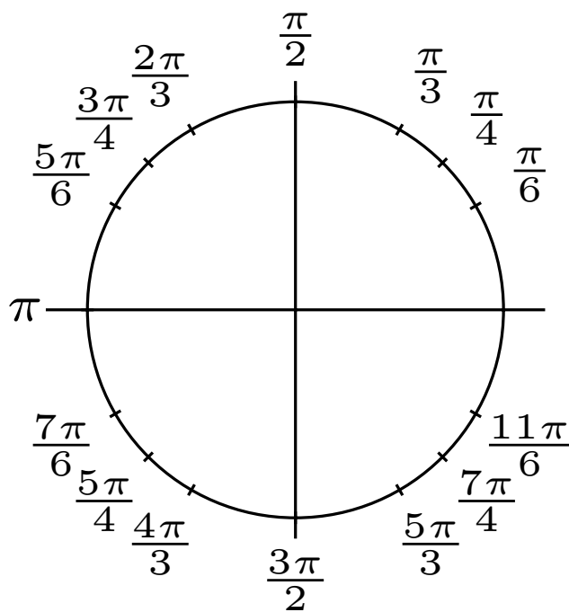
Figure 18 The Unit Circle with Important Angles
