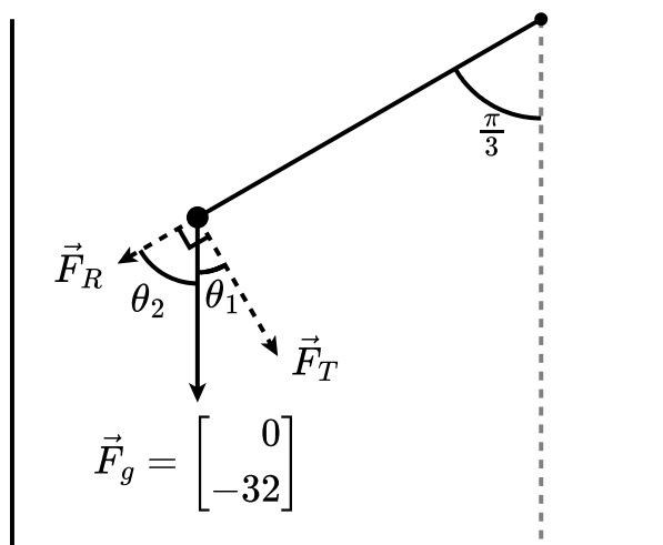
Figure 64 Force Vectors Acting on a Pendulum
