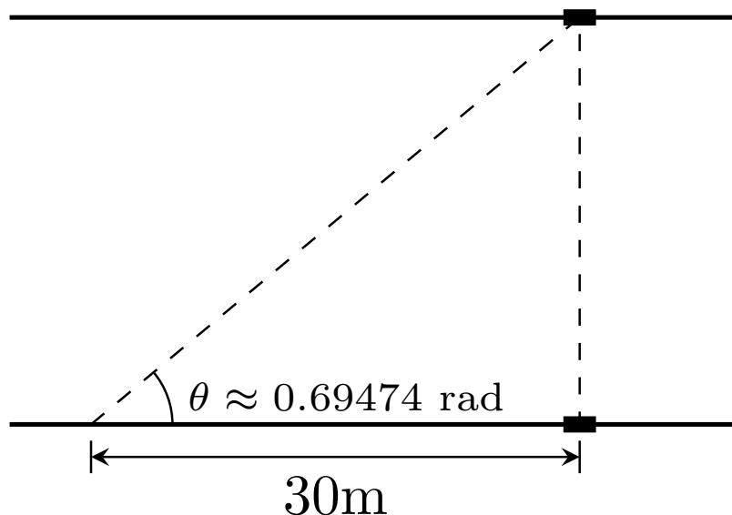
Figure 25 Two Gatehouses on a Canal Lock
