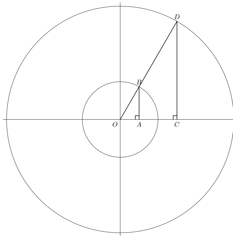
Figure 23 Circles with Similar Triangles
