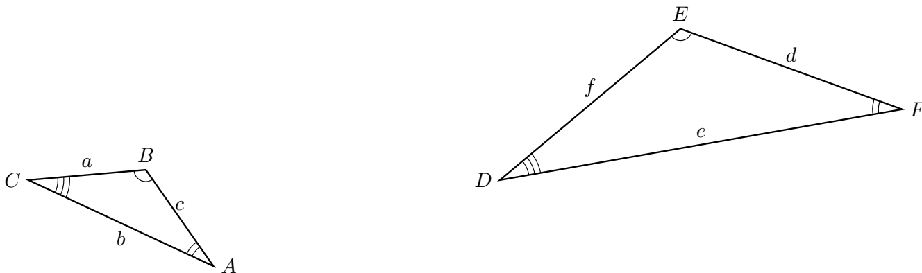
Figure 20 An Example of Similar Triangles
