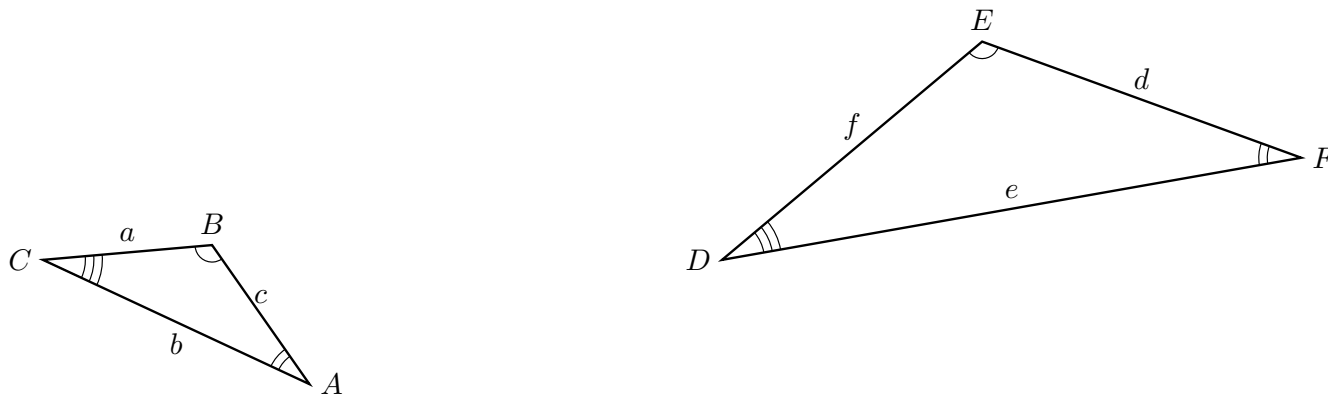
Figure 17 An Example of Similar Triangles
