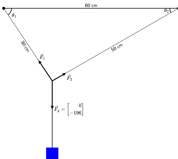
Figure 61 A Weight Suspended Asymmetrically
