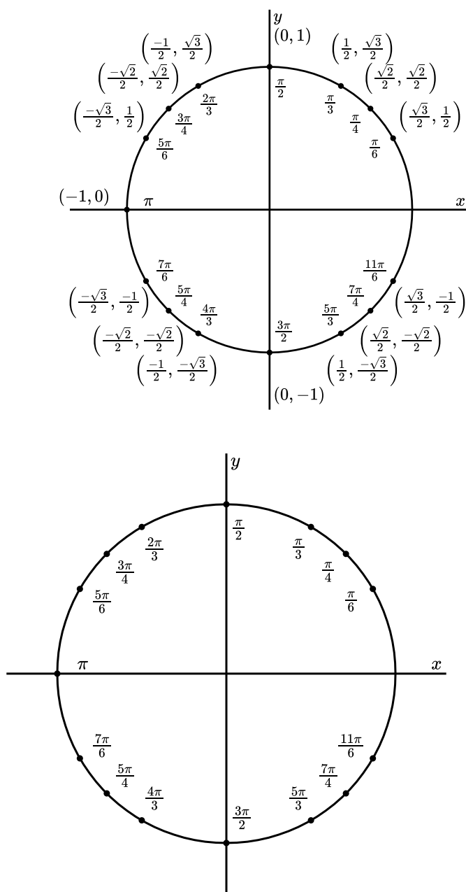
Figure 17 The Unit Circle with Important Angles
