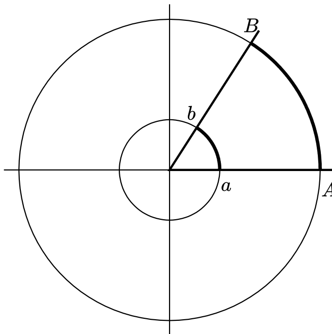
Figure 13 One radius of arc length on two different circles
