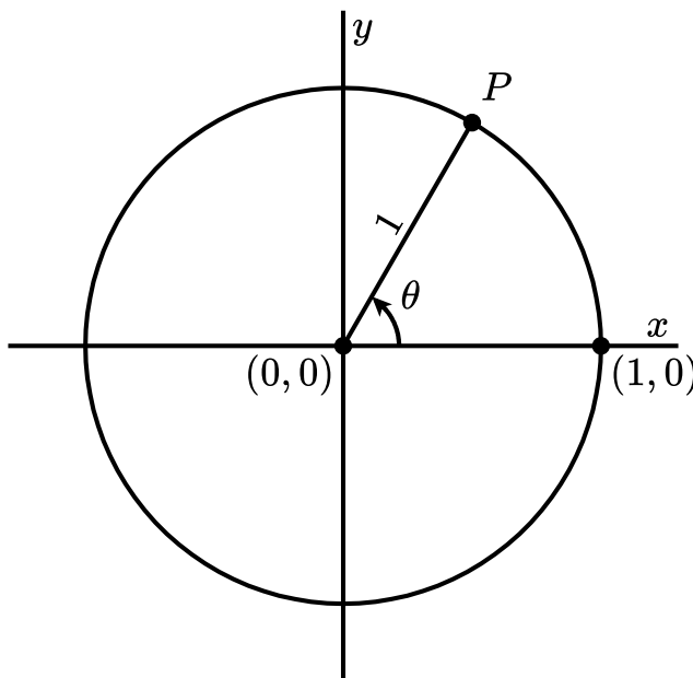
Figure 14 The Unit Circle with an Angle Shown
