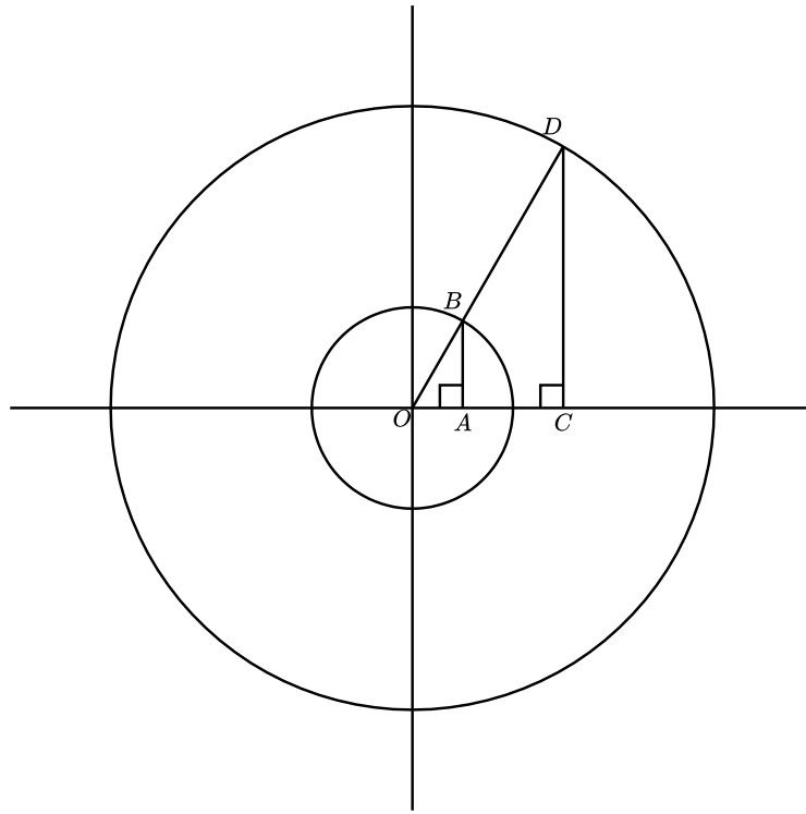
Figure 22 Circles with Similar Triangles
