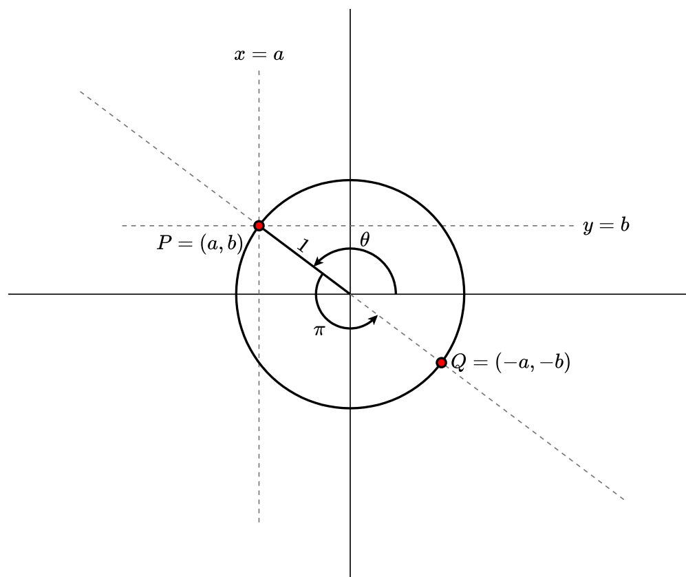
Figure 30 The unit circle showing \cos(\theta) , \sin(\theta) , and \tan(\theta) .
