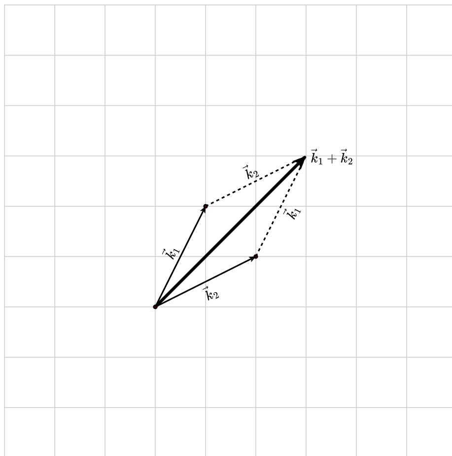
Figure 11 Adding Vectors Graphically.
