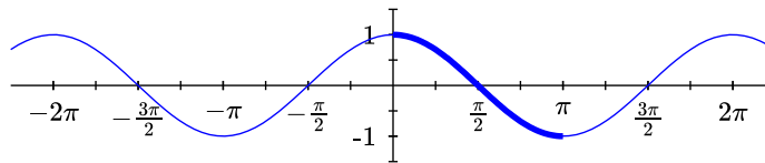
Figure 48 The Cosine Function and its Principle Branch
