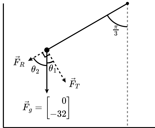
Figure 71 Force Vectors Acting on a Pendulum
