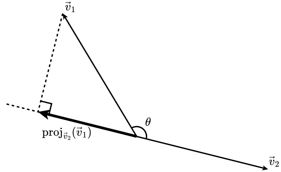
Figure 59 Orthogonal Projection of \vec{v}_1 onto \vec{v}_2
