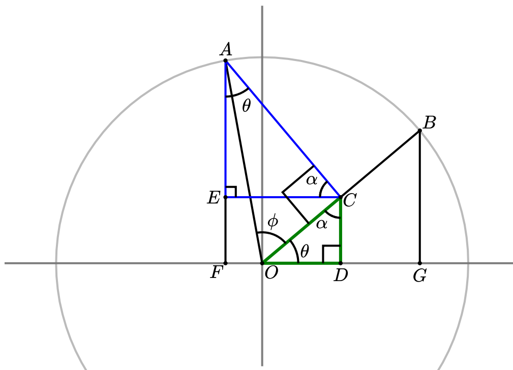
Figure 50 The Unit Circle with Points at Angles \theta and \theta + \phi
