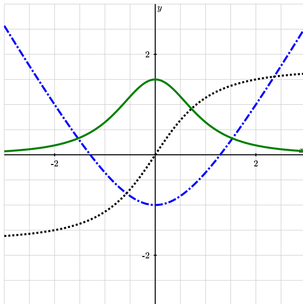
Figure 3.9.1 The graphs y = \ell(x) , y = M(x) , and y = k(x) .
