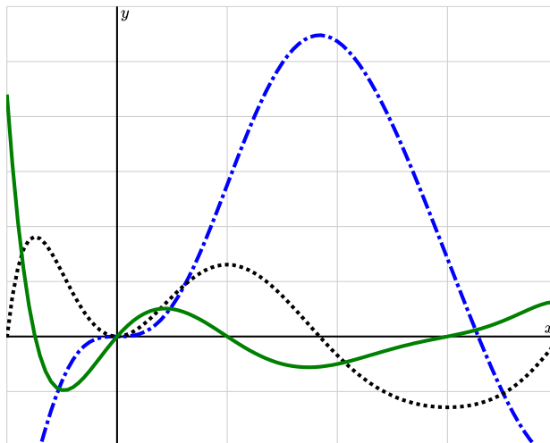
Figure 3.9.2 The graphs y = h(x) , y = T(x) , and y = s(x) .
