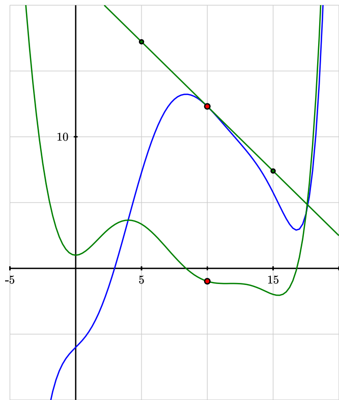
Figure 7 The graph of f(x) and the tangent line at a = 10 .
