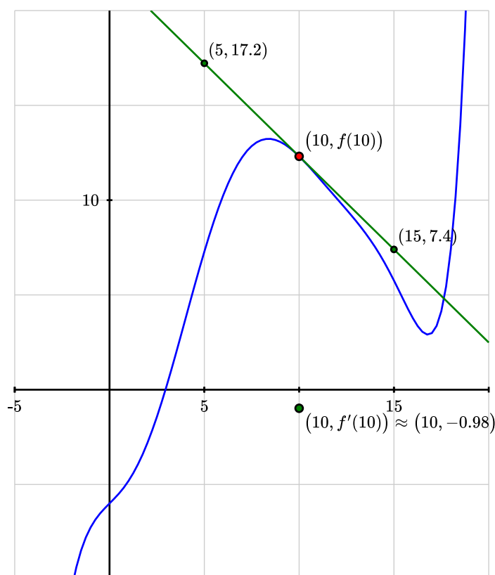
Figure 6 The graph of f(x) and the tangent line at a = 10 .
