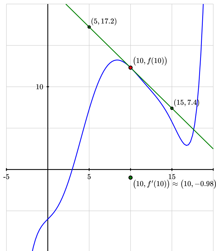
Figure 3.6.1 The graph of f(x) and the tangent line at a = 10 .
