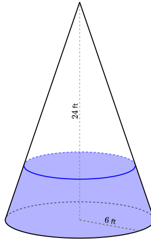
Figure 6.1.1 A Conical Tank with Base Radius 6 ft and Height 24 ft.
