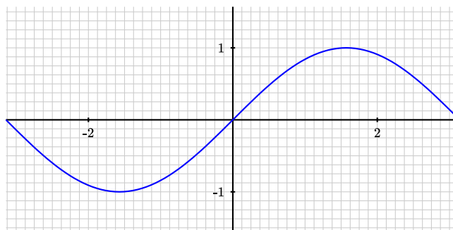
Figure 3.11.6 The graph of y = g(x)
