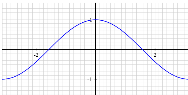
Figure 3.11.5 The graph of y = f(x)
