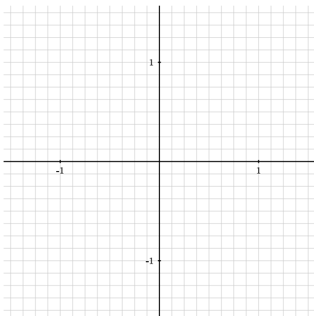
Figure 3.11.3 A Blank Grid for Drawing y = f'(x)
