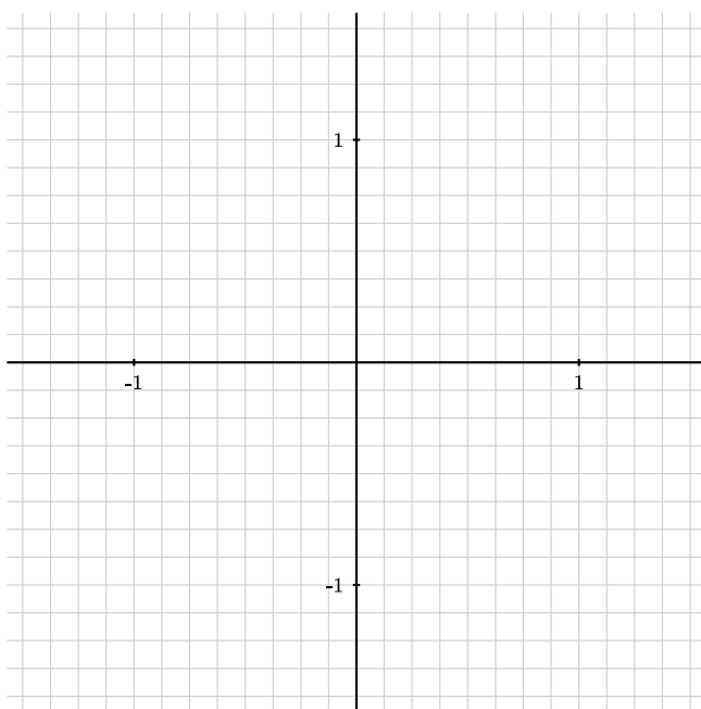
Figure 3.11.4 A Blank Grid for Drawing y = g'(x)
