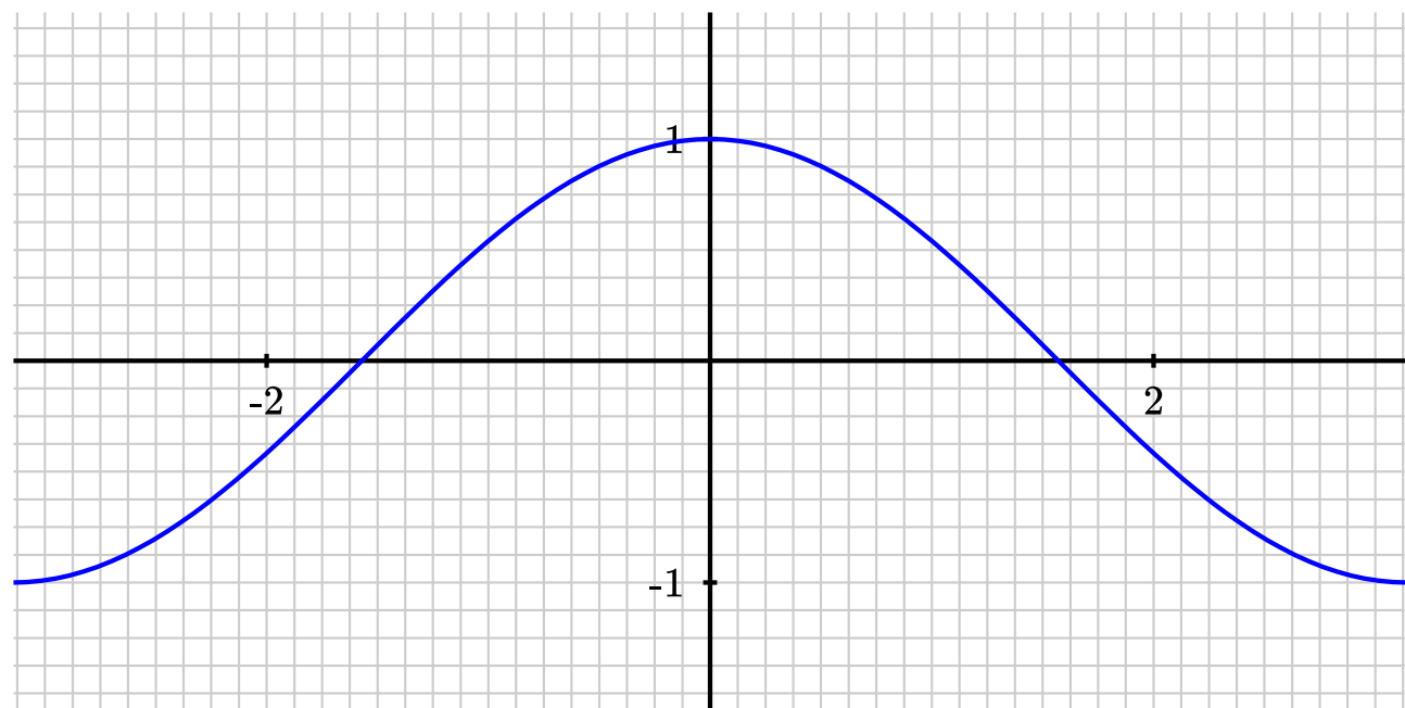
Figure 3.11.3 The graph of y = f(x)
