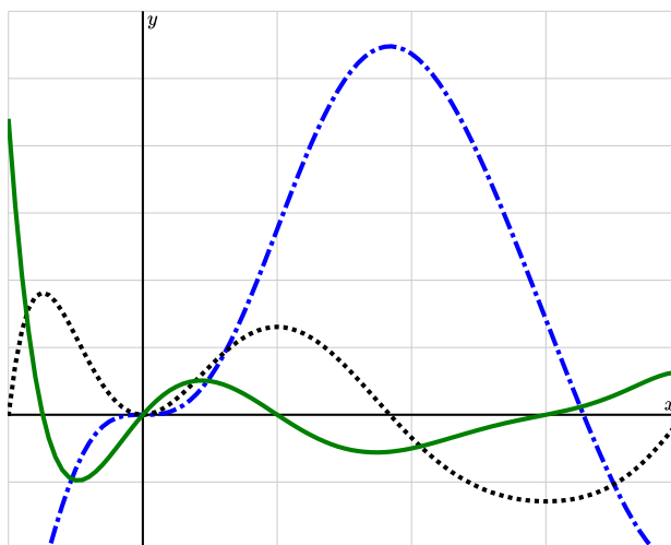
Figure 3.10.2 The graphs y = h(x) , y = T(x) , and y = s(x) .
