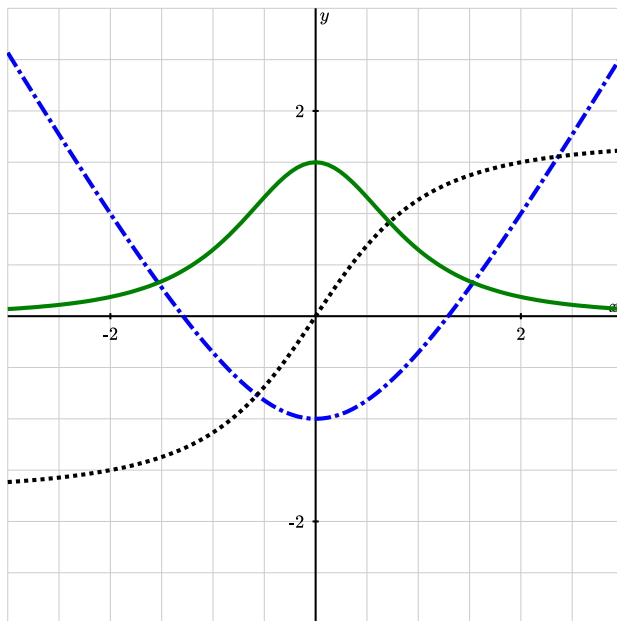
Figure 3.10.1 The graphs y = \ell(x) , y = M(x) , and y = k(x) .
