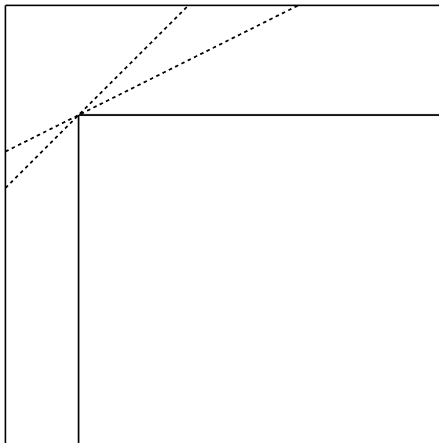
Figure 3.12.1 Two Hallways and Possible “Ladders”
