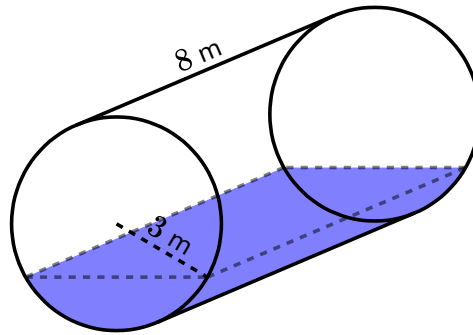
Figure 6.1.3 A Cylindrical Tank with Radius 3 m and Length 8 m.
