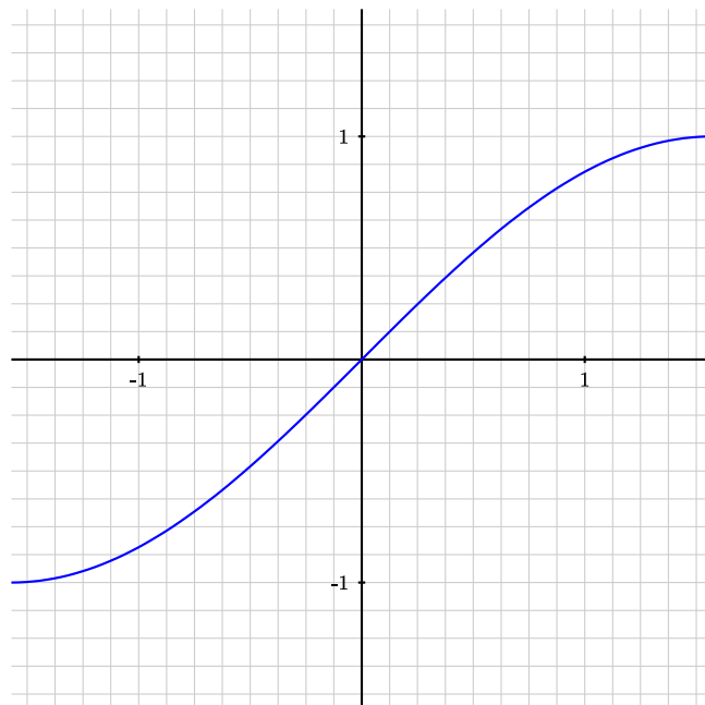
Figure 3.11.2 The graph of y = g(x)
