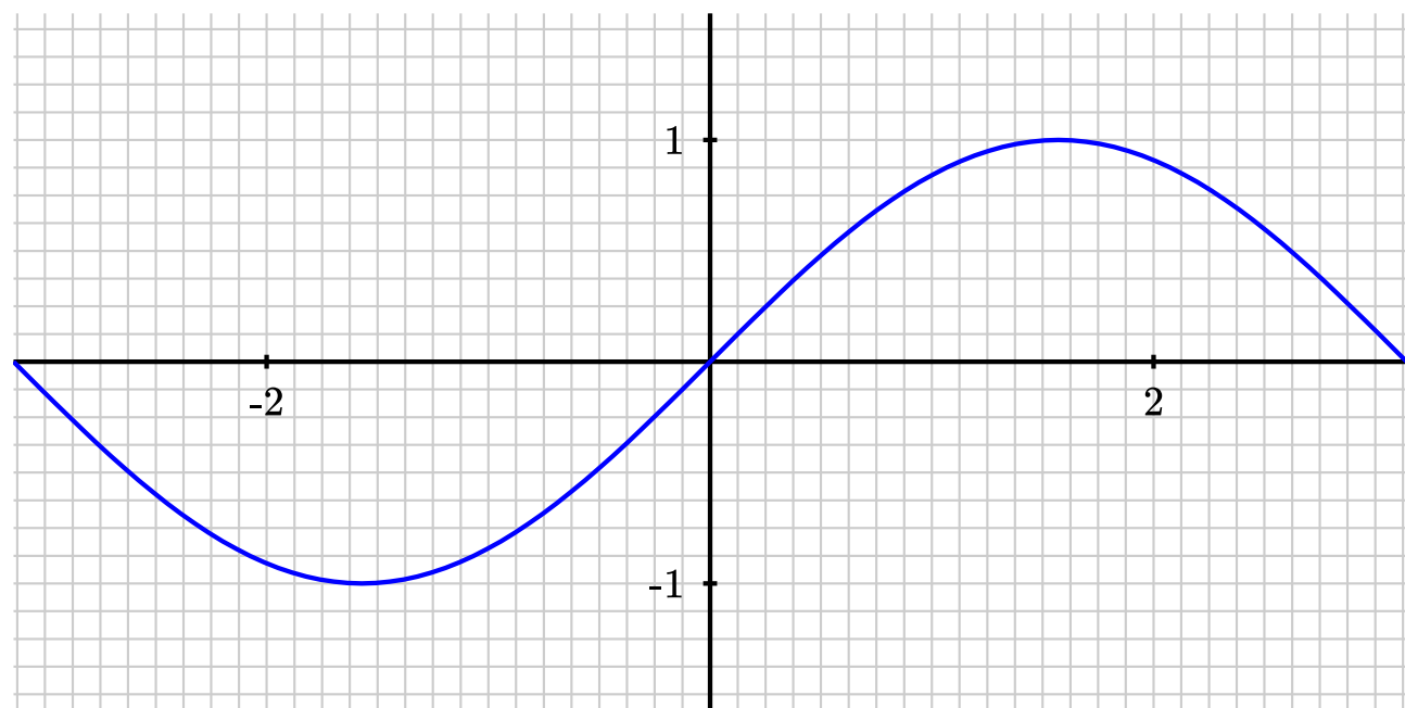
Figure 3.11.4 The graph of y = g(x)
