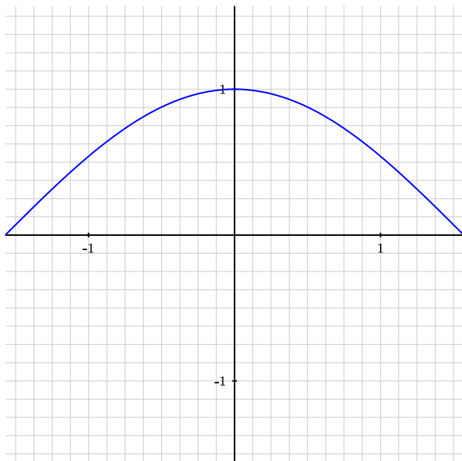
Figure 3.11.1 The graph of y = f(x)
