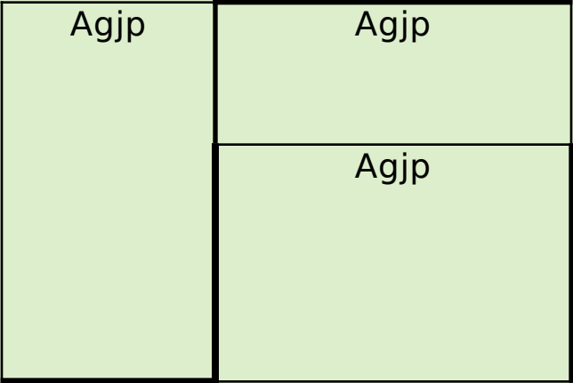
vertical-merge-conflicting
