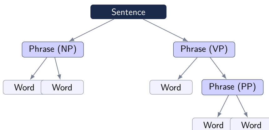
Figure 4.1: Illustrative RLE tree: a Sentence root decomposes recursively into Phrase and Word nodes.
