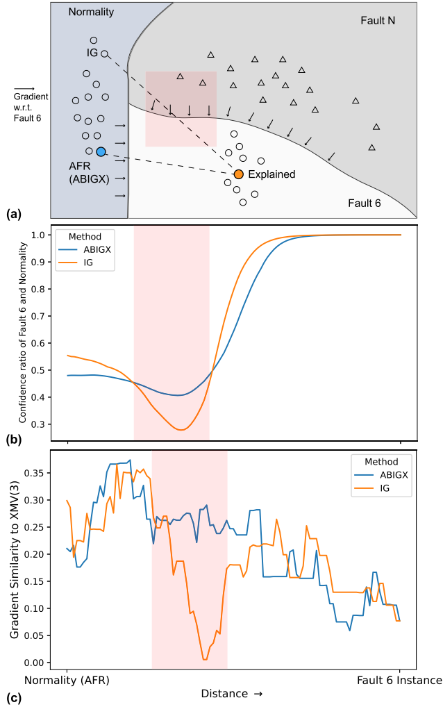
Fig. 4. Comparison of ABIGX and Vanilla IG explanations for TEP [18] fault classification model. (a) The intuitive illustration (not the real cases) of two baselines and integral paths on model boundary; (b) The model confidences along the two paths from two baselines to explained sample; (c) The cosine similarity between gradient direction and the root variable XMV(3), along the same paths. The red boxes in three figures are noisy areas corresponding to each other.
