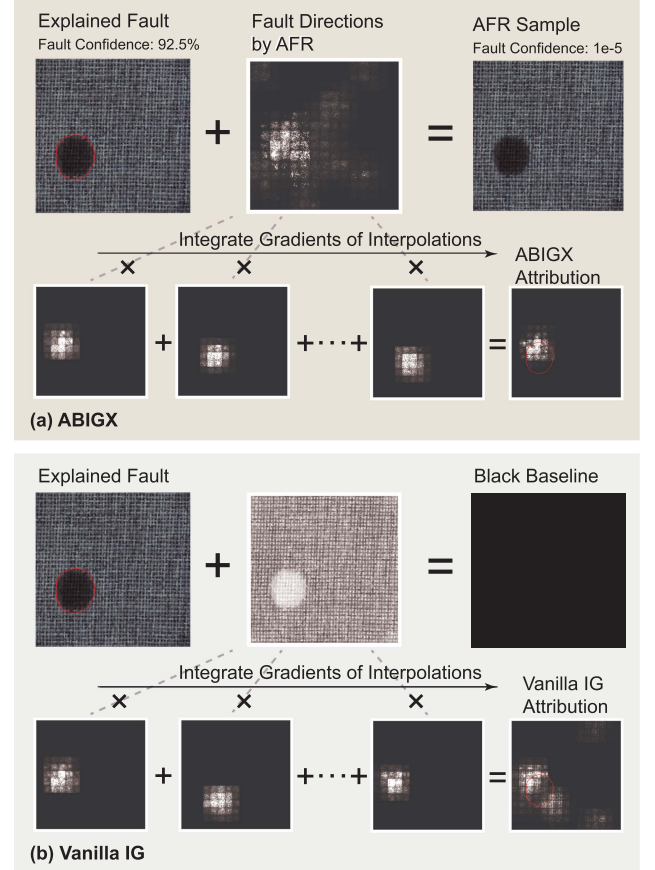
Fig. 3. Comparison of ABIGX (a) and Vanilla IG (b) explanations for the Win-Clip [32] model using an anomaly image from MVTec-AD [33]. ABIGX differs by using AFR to adaptively find a semantically meaningful, fault-suppressing baseline, leading to more informative path gradient integration.
