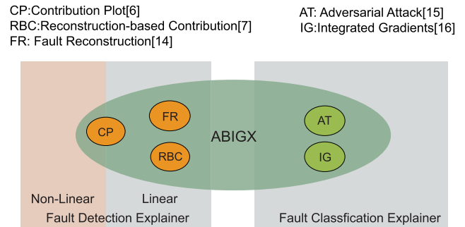
Fig. 1. The illustration of ABIGX and related methods. ABIGX is an explanation framework applicable for both linear and non-linear fault detection and classification models. It frames two classical fault diagnosis methods (CP and RBC) and generalizes to general FDC models aided by adversarial attack and IG method.
