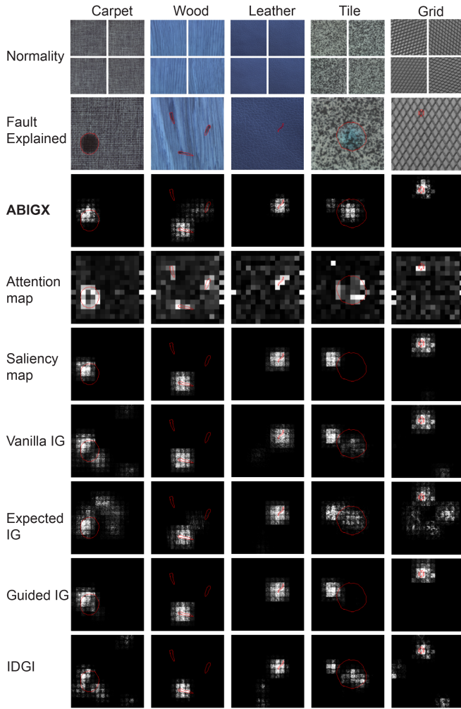
Fig. 8. Explanation results for the WinClip anomaly detector on five samples from the MVTec-AD dataset. Ground-truth anomaly regions are circled in red (zoom in to view finer details in small regions).
