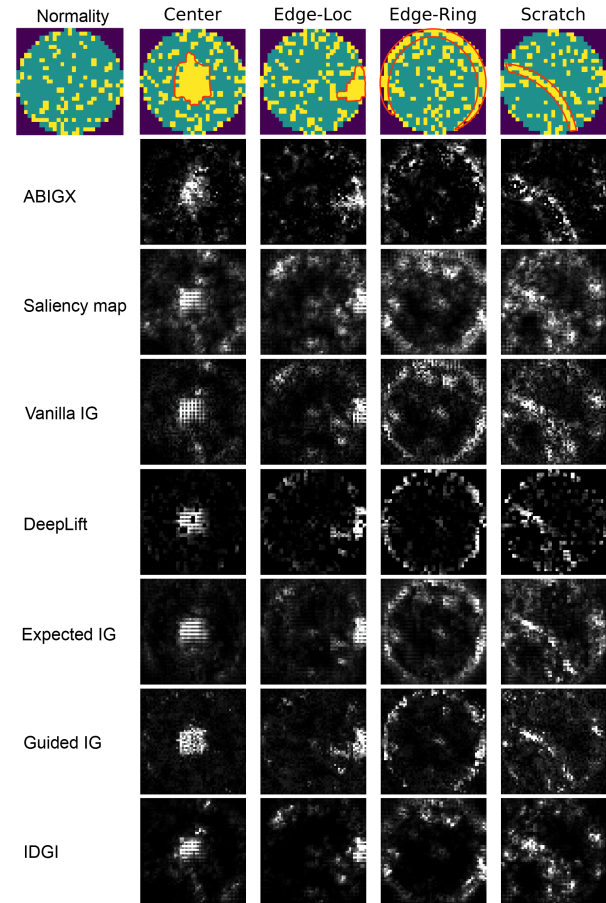
Fig. 7. Explanations for CNN classifier on four sampled wafer maps with different fault patterns, where the ground-truth root pixels are circled in red.
