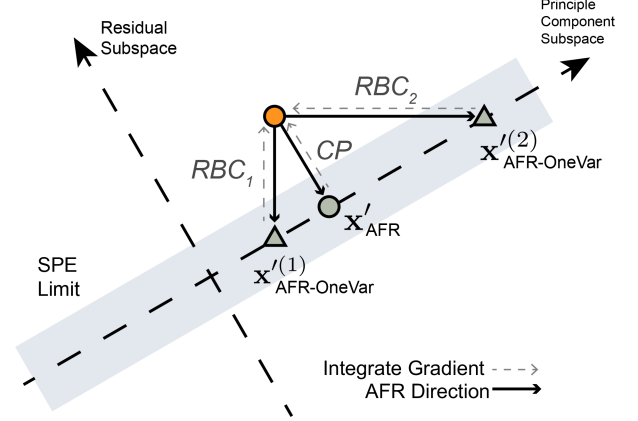
Fig. 5. Illustration of ABIGX on 2-D PCA-based detection: CP is identical to the integrated gradients between the explained sample and \mathbf{x}'_{AFR} ; RBC is identical to the integrated gradients between the explained sample and \mathbf{x}'_{AFROV} on each variable direction.
