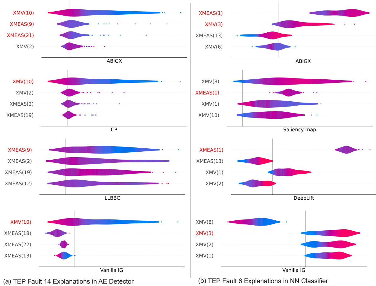
Fig. 6. Explanations comparison for the NN classifier on TEP Fault 6, where the ground-truth root variables are in red. Fault 6 is caused by root variables XMEAS(1) and XMV(3) and Fault 14 is caused by XMEAS(9), XMV(10), and XMEAS(21), detailed in Table B.2.
