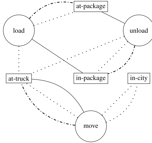
Fig. 1. LDMG for the simplified Logistics original domain model. Dotted lines indicate preconditions, dashed lines indicate negative effects, and full lines indicate positive effects. For the sake of readability, we represent operators by circles and predicates by rectangles as well as we omit variables for the same reason.
