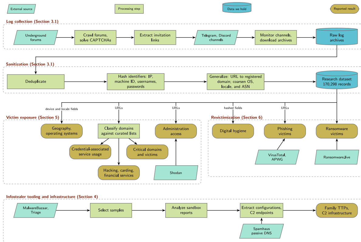
Fig. 1. Pipeline of our methodology, from acquiring malware logs from illicit sources to the analyses each section reports.
