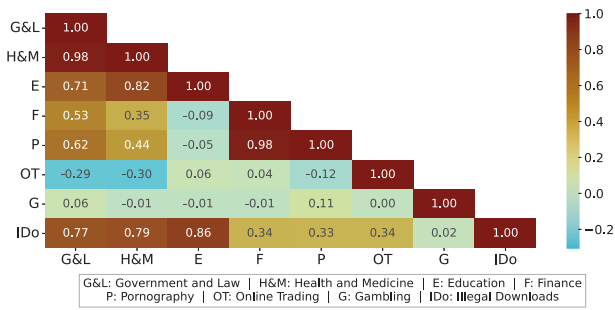
Fig. 6. Cosine similarity between the categories of credential-associated service usage, under strict filtering (>500 domains per victim, \geq 200 victims per category; n = 322 victims).
