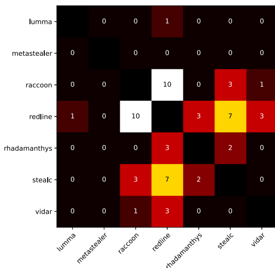
Fig. E.1. Common infrastructure used as C2 servers by different infostealers.
