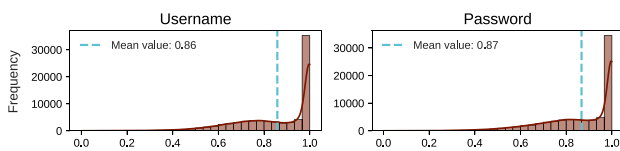
Fig. 10. Statistics on credential leakage, filtered to include only victims with 50 or more credentials.
