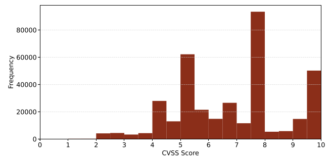
Fig. 8. CVSS distribution of vulnerabilities.
