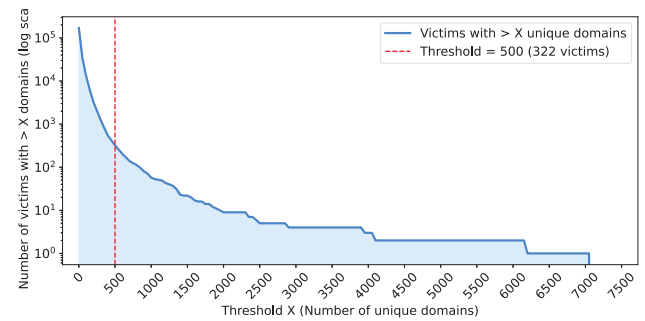
Fig. 5. Number of victims with strictly more than X unique domains, plotted on a logarithmic scale. The red dashed line marks the analytical threshold of \geq 500 unique domains ( n = 322 victims). (For interpretation of the references to color in this figure legend, the reader is referred to the web version of this article.)
