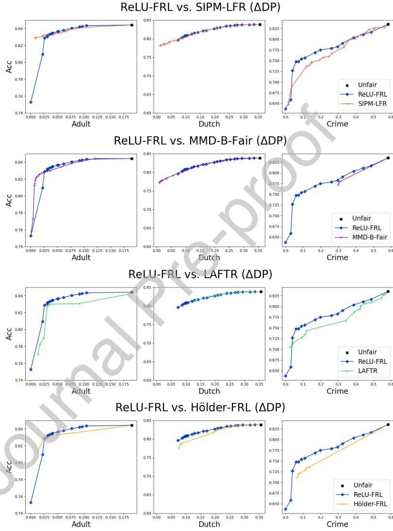
Figure D.6: Single-layered NN prediction head: Pareto-front lines of fairness level \Delta DP and ACC. (Left) ADULT, (Center) DUTCH, (Right) CRIME.
