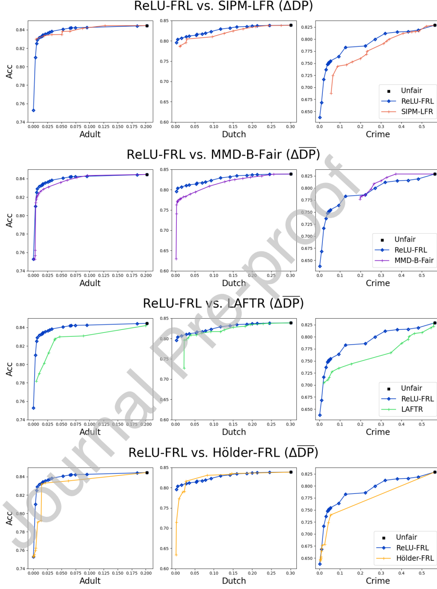
Figure 1: Linear logistic prediction head: Pareto-front lines of fairness level \Delta\overline{DP} and ACC. (Left) ADULT, (Center) DUTCH, (Right) CRIME.
