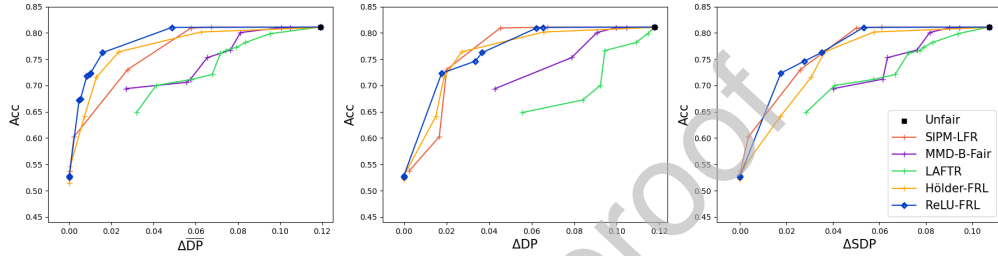
Figure 2: Pareto-front lines on CELEBA of fairness level ( \Delta\overline{DP} , \Delta DP , \Delta SDP ) and ACC.
