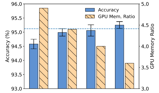
Fig. 10. Tradeoffs between GPU memory efficiency and accuracy in STDL. The dashed line denotes BPTT's accuracy. GPU memory ratio is the memory of BPTT divided by that of STDL.
