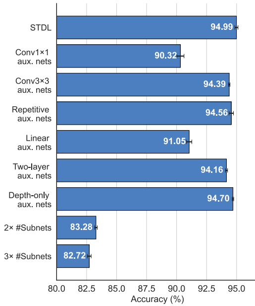
Fig. 9. Influences of auxiliary networks and subnetworks. Each row denotes a variant of STDL with a modification described on the y-axis. The blue bar chart reports each variant's accuracy for ResNet-18 on CIFAR-10.
