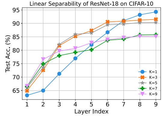
Fig. 3. Comparison of layer-wise linear separability among supervised local learning variants that evenly divide ResNet-18 into K subnetworks.
