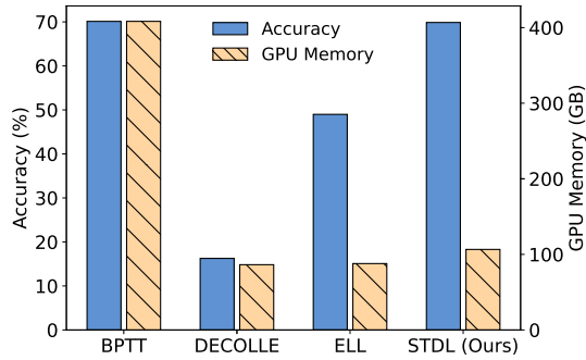
Fig. 1. Comparison of BPTT, supervised local learning rules (DECOLLE and ELL), and the proposed STDL method in terms of accuracy and GPU memory for training the SEWResNet-34 network on the ImageNet dataset.
