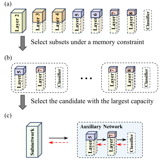
Fig. 4. Illustration of auxiliary network construction in STDL. For each subnetwork, the auxiliary network is constructed by selecting a subset of its subsequent layers. The subnet has the largest expressive capacity, i.e., depth and width, while not exceeding a given memory constraint. The shaded area within each layer represents its memory footprint during training. (a) Subsequent layers. (b) Auxiliary network candidates with the greatest depth. (c) Constructed auxiliary network and its subnetwork.
