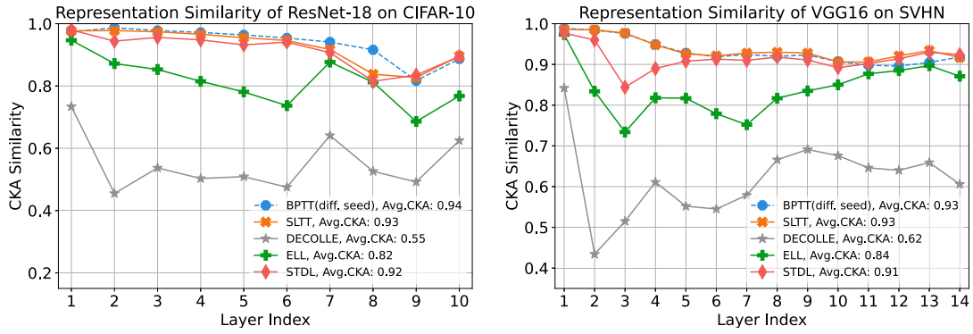
Fig. 7. Comparison of layer-wise representation similarity. We utilize CKA [69] to measure the layer-wise similarity of representations between BPTT and other learning rules. To provide a fair baseline for BPTT, we measure the similarity between two networks trained with different random seeds. The average CKA similarity scores over all layers for different learning rules are provided in the legend.
