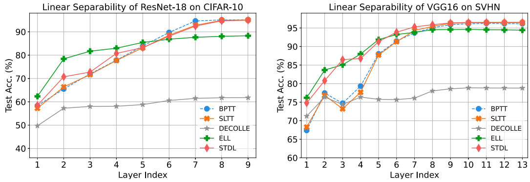
Fig. 8. Comparison of layer-wise linear separability among STDL and baselines.
