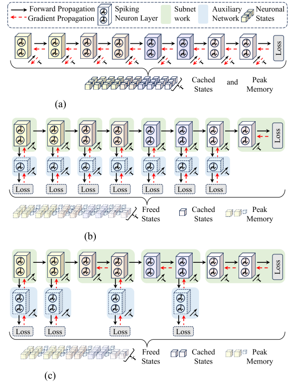
Fig. 2. Comparison of BPTT, supervised local learning, and our STDL for training SNNs. (a) BPTT caches the entire trajectory of neuronal states during forward propagation for gradient computation, with memory overhead scaled along with both the number of layers and time steps. (b) Supervised local learning caches the states of only one layer at each time step, as it enables the online learning of each network layer along with an auxiliary linear classifier independently. (c) STDL partitions the original network into subnetworks by grouping as many adjacent layers as possible without affecting the peak memory. Each subnetwork is independently trained with an auxiliary network in an online learning manner. For both (b) and (c), once the forward propagation of a subnetwork and its auxiliary network is completed, their gradients are immediately calculated, followed by freeing the cached states.
