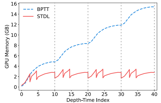
Fig. 6. GPU memory usage pattern with respect to the layer and time index. ResNet-18 is trained with BPTT and STDL on CIFAR-10 with four steps.
