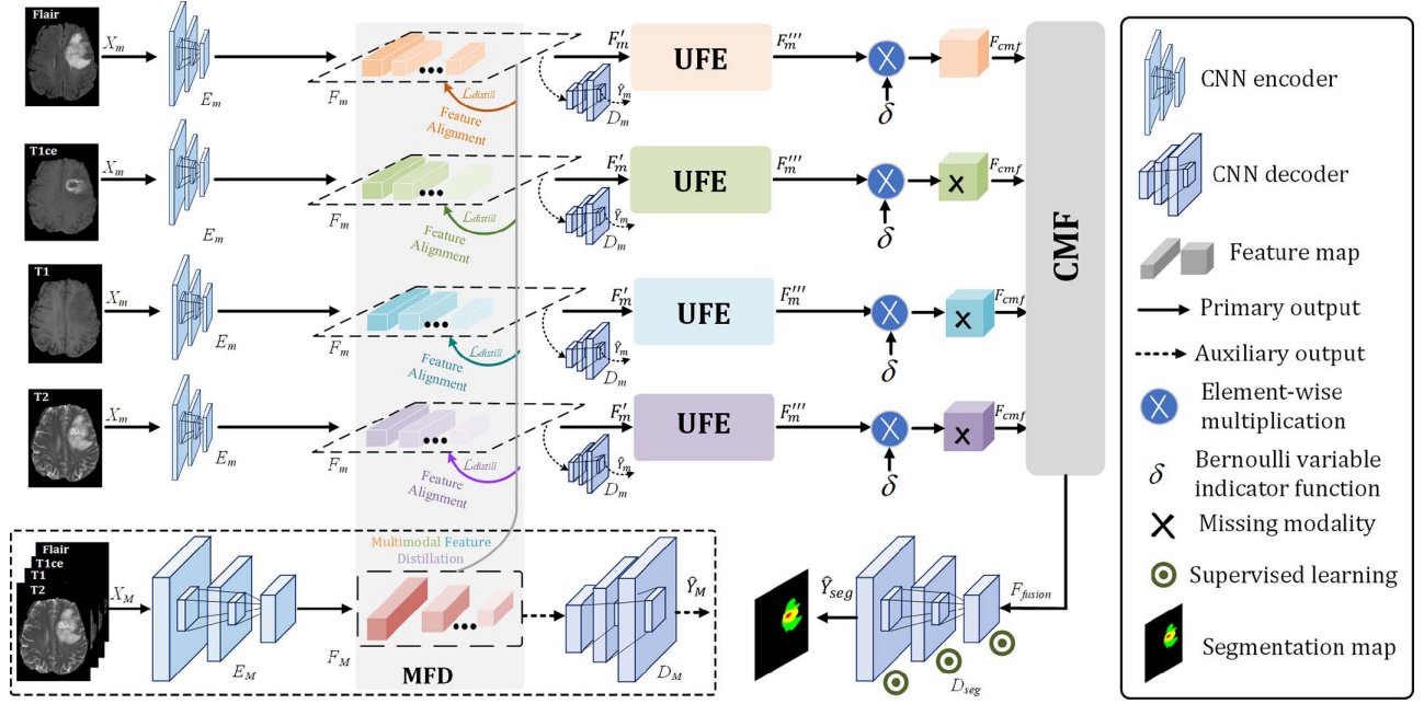
Fig. 2. Overview of the proposed model. The MFD module adopts a multimodal encoder network to distill complementary multimodal knowledge into the unimodal encoders. The UFE module extracts intra-modal feature maps. The CMF module is then used to aggregate features across modalities. D_{seg} produces the final segmentation result \hat{Y}_{seg} . The auxiliary outputs \hat{Y}_m of D_m and \hat{Y}_M of D_M are used in loss functions along with the segmentation map of the primary output. The description of symbols in the figure is given in the legend box.
