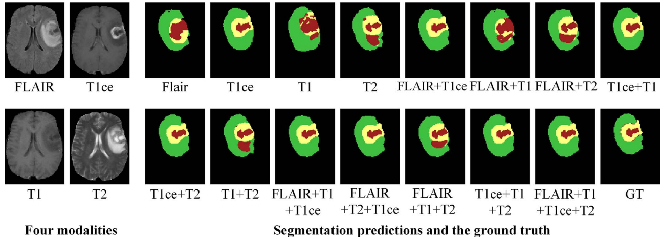
Fig. 5. Qualitative comparison for segmentation results of fifteen different missing modalities. Four different modalities are on the left, and segmentation results and ground truth of the proposed model are in fifteen different combinations on the right.
