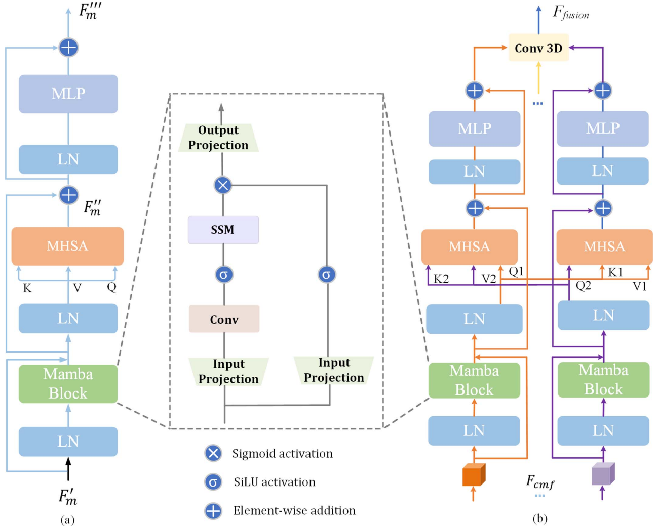
Fig. 3. Structure of: (a) UFE and (b) CMF. The structure of the Mamba block contains the projection layer, the SSM, the convolutional layer, and sigmoid linear unit (SiLU) activation functions, which are in the middle of the figure shared with UFE and CMF.
