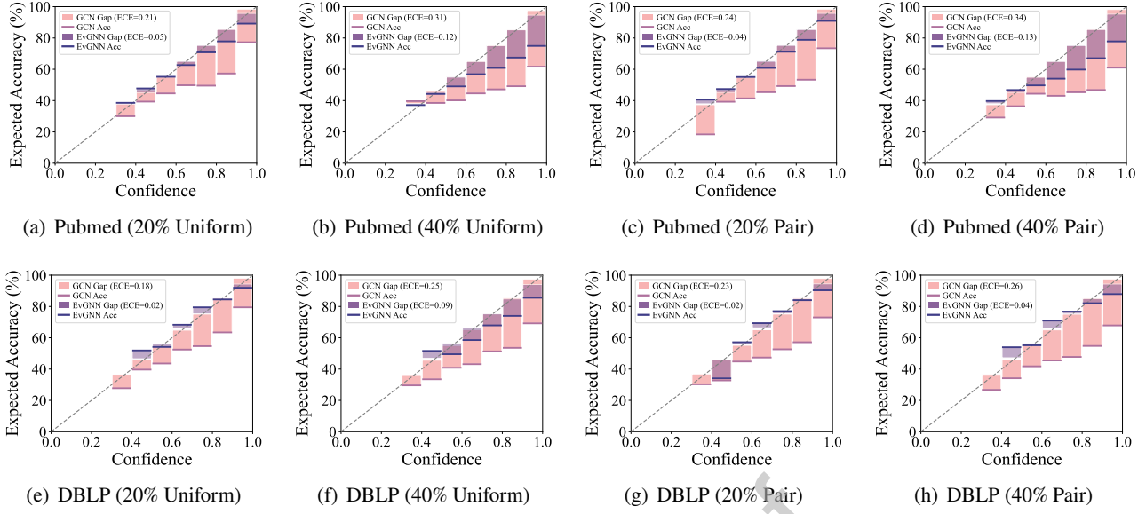
Figure 7: Comparison of calibration gaps and ECE on Pubmed and DBLP.
