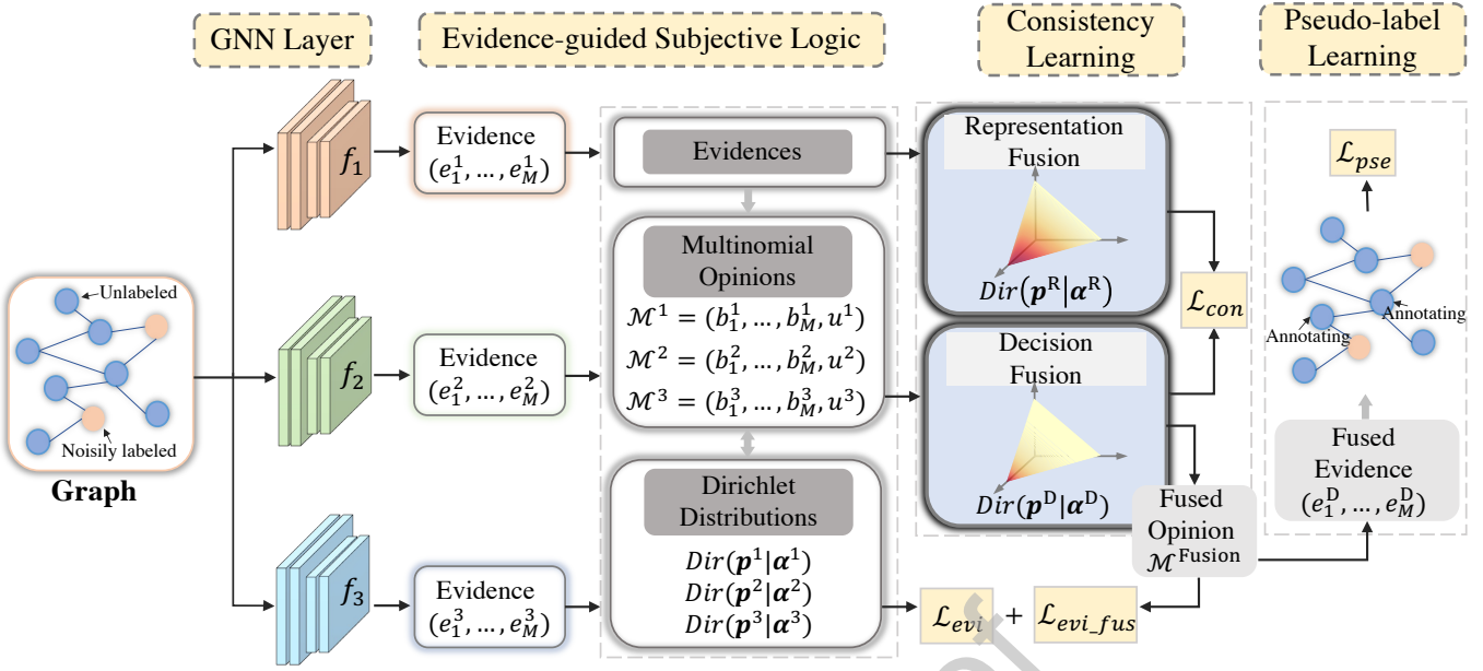
Figure 2: Framework overview of the proposed method EvGNN.
