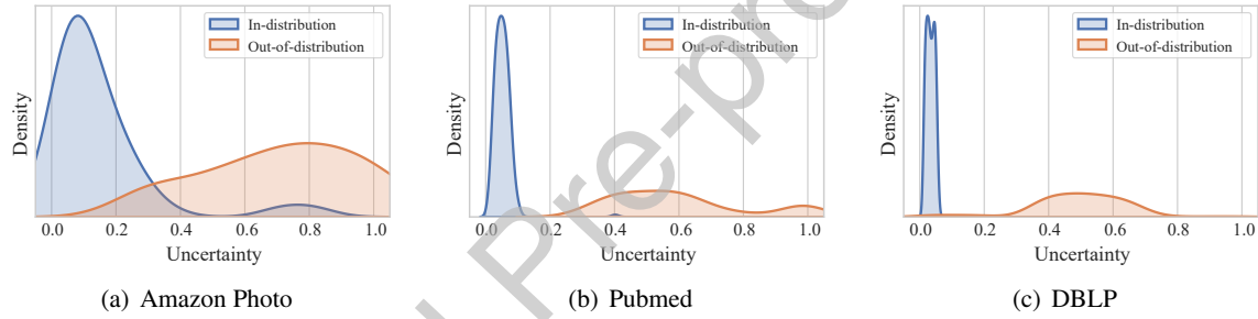
Figure 8: Distributions of uncertainty for in-distribution and out-of-distribution data on Amazon Photo, Pubmed, and DBLP.
