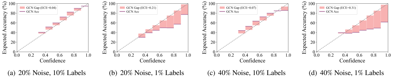
Figure 1: Motivating experiment on Pubmed under uniform label noise and sparse supervision. ECE measures the discrepancy between prediction confidence and empirical accuracy, where a lower value indicates better calibration.
