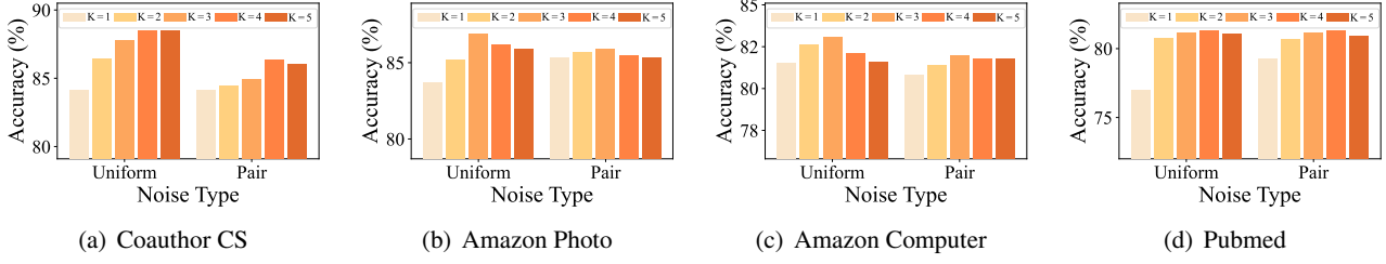
Figure 6: Sensitivity analysis w.r.t. expert number K on Coauthor CS, Amazon Photo, Computer, and Pubmed.
