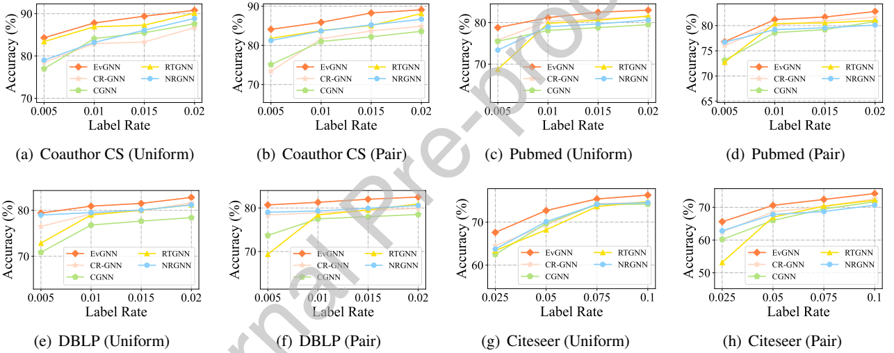
Figure 4: Comparison w.r.t. different label rates on Coauthor CS, Pubmed, DBLP, and Citeseer.
