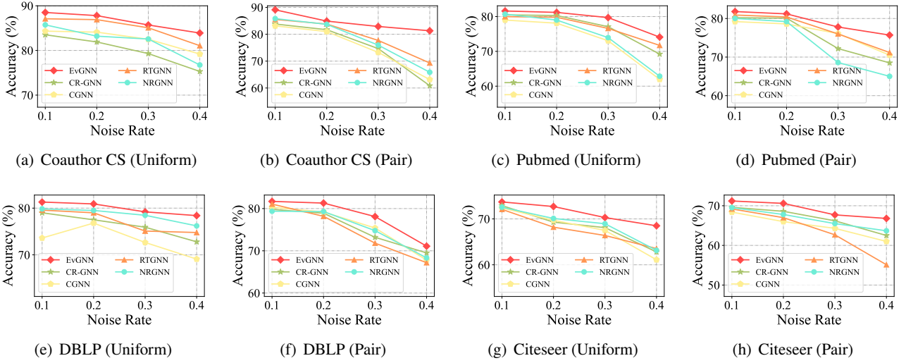
Figure 3: Comparison w.r.t. different noise rates on Coauthor CS, Pubmed, DBLP, and Citeseer.
