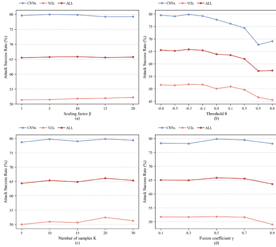
Fig. 4. Ablation study of the scaling factor \beta , threshold \theta , number of samples K , and fusion coefficient \gamma .
