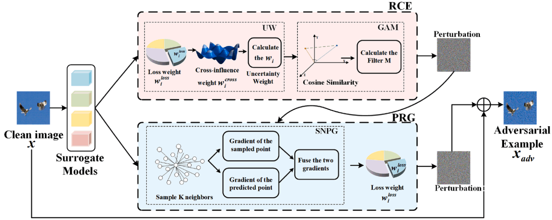
Fig. 2. An overview of FUGEA. The gradient obtained from the surrogate model is optimized through the RCE and PRG stages to generate adversarial examples with strong cross-architecture transferability.
