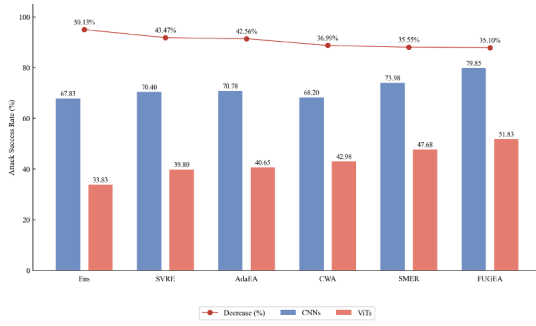
Fig. 1. A comparison of the adversarial attack transferability of adversarial examples generated by FUGEA and baseline methods through ensemble training on ResNet18, Inception_v3, BiT-M-R50 \times 1, and Inception_v4. Our FUGEA achieves the best performance by optimizing ensemble gradients with a two-stage strategy.
