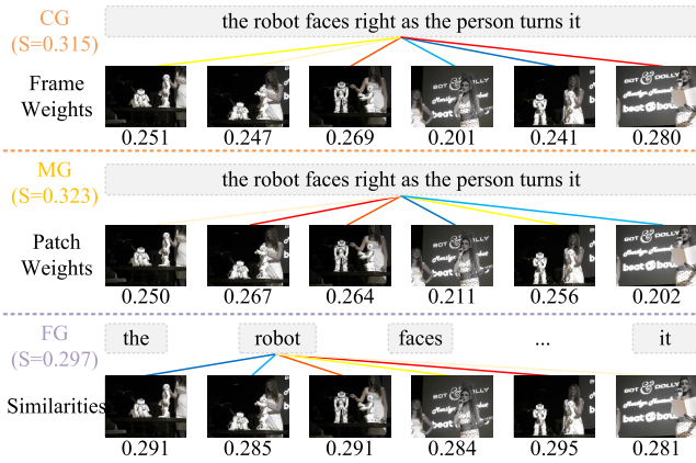
Fig. 10. Visualization of the weight and similarity values in the coarse-to-fine interaction. The weight and similarity are represented in the following colors from high to low: red, light red, yellow, light yellow, blue, and light blue, respectively.
