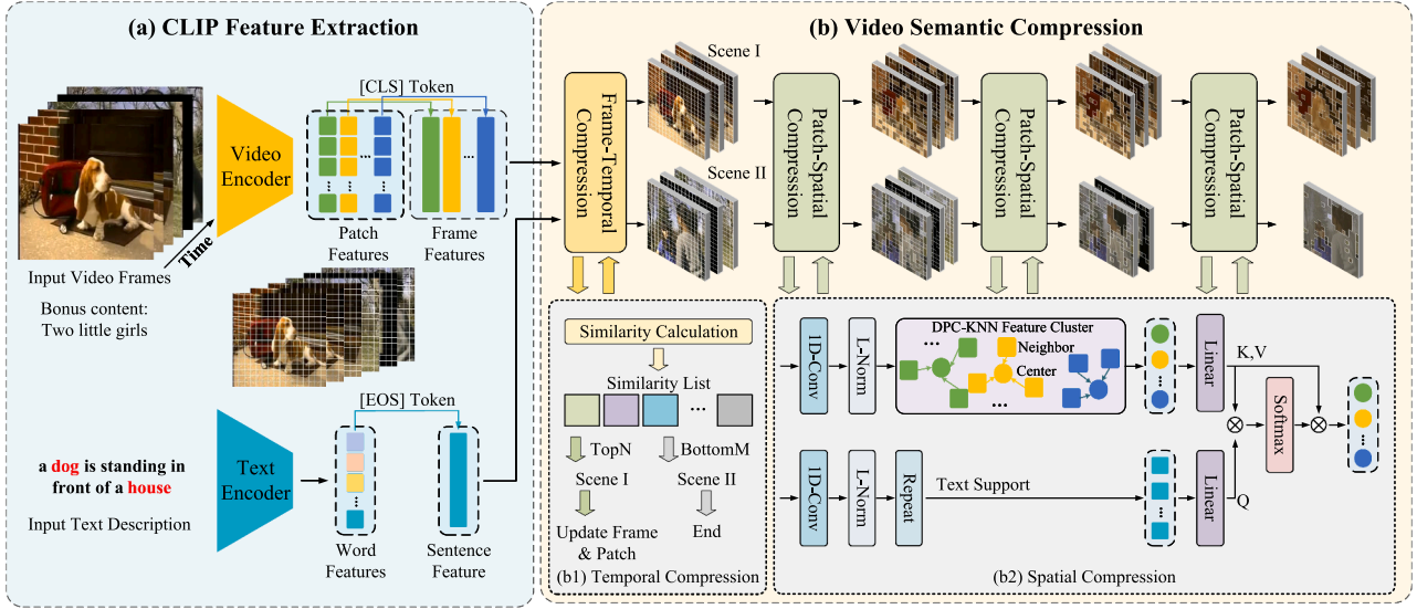
Fig. 2. Framework. (a) The CLIP Feature Extraction module leverages CLIP (Radford et al., 2021) to extract both text features (sentence and words) and video features (frames and patches). (b) The Video Semantic Compression module includes (b1) temporal-level frame compression and (b2) spatial-level patch compression. \otimes denote matrix multiplication.
