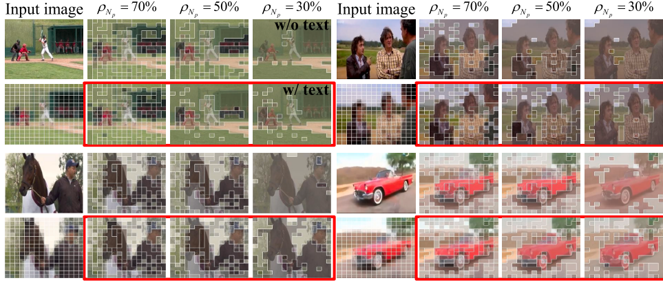
Fig. 9. Visualization of patch compression with text support. The red box (w/ text) indicates the results obtained with textual guidance.
