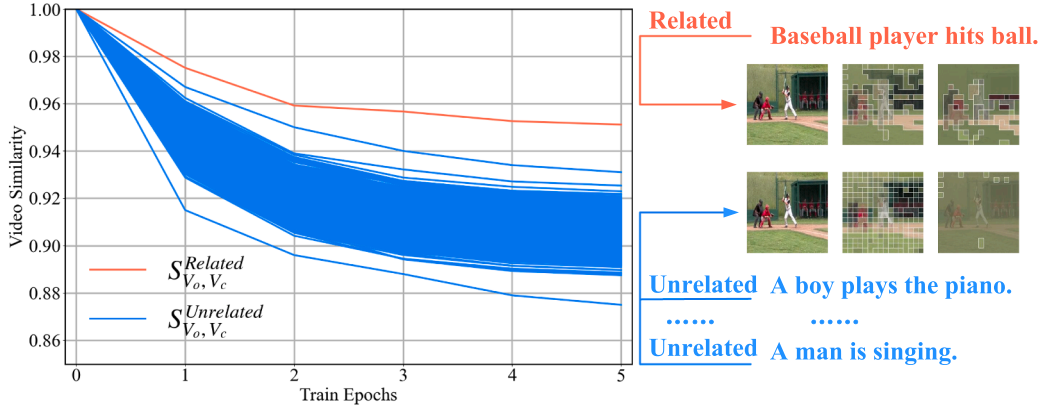
Fig. 3. Similarity. Video similarity before and after compression. We select video7021 as an example to compare the video similarity before and after compression under 1000 different text conditions. The similarity for the related text-video pair S_{V_o, V_c}^{Related} is marked in red, while that for the 999 unrelated text-video pairs S_{V_o, V_c}^{Unrelated} is marked in blue.
