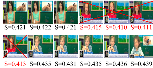
Fig. 7. Visualization of the video frame selection process. Given a query text and sampled video frames, the frames with the highest similarity scores are retained.
