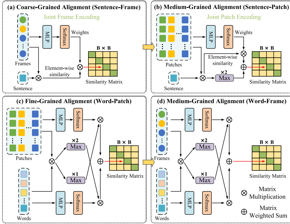
Fig. 4. Framework. (a) Coarse-grained interaction between a text sentence and a video frame features. (b) Medium-grained interaction between text sentence and video patch features. (c) Fine-grained interaction between sentence words and video patch features. (d) Medium-grained interaction between sentence words and video frame features. \oplus and \otimes denote matrix addition and multiplication, respectively.
