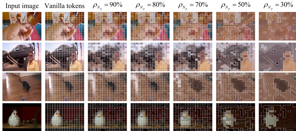
Fig. 8. Visualization of the frame patch compression process. \rho_{N_p} denotes the ratio of the number of features after compression to that before compression.
