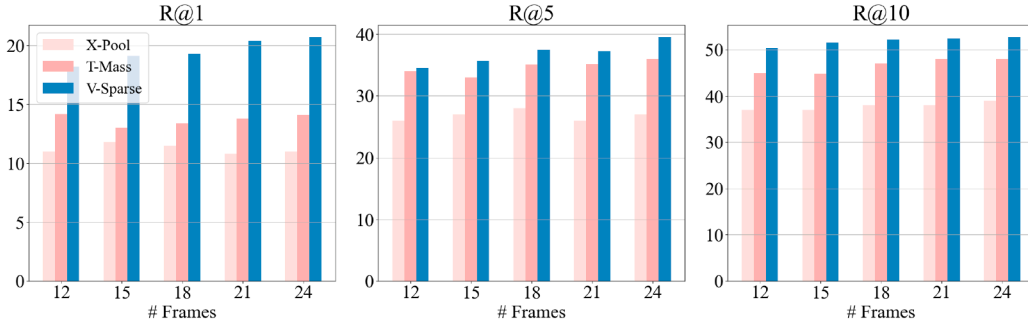
Fig. 5. Ablation of different sampling frame numbers on the Charades (Sigurdsson et al., 2016).
