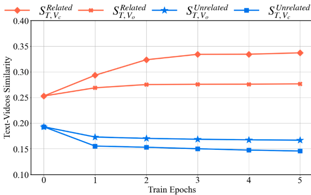
Fig. 6. Text-video similarity. The similarities between the related and unrelated text-video pairs are denoted by S_{T,V}^{Related} and S_{T,V}^{Unrelated} , respectively. A larger S_{T,V}^{Related} is better, while a smaller S_{T,V}^{Unrelated} is better. The representations of V include both the original visual feature V_o and the compressed visual feature V_c .
