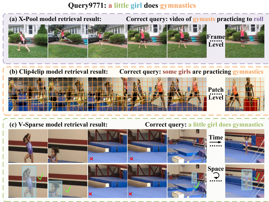
Fig. 1. Motivation. Taking query9771 as an example, we illustrate the limitations of existing model under sparse text and redundant visual features. (a, b) Failed retrieval results from the frame-based feature enhancement model X-Pool (Gorti et al., 2022) and the patch-based feature interaction model Clip4clip (Luo et al., 2022). (c) Successful retrieval results from our model V-Sparse, which benefits from text-supported temporal-spatial visual semantic compression and adaptive coarse-to-fine feature interaction.
