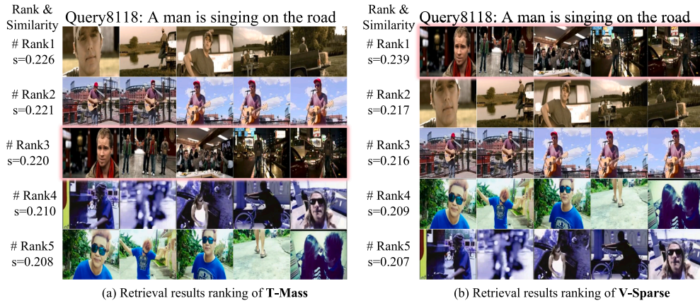
Fig. 12. Visualization of T-Mass and V-Sparse retrieval results. The ground-truth result is highlighted in pink, and the ranking is based on similarity scores.
