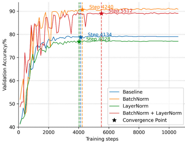
Fig. 7. Impact of BN & LN on performance.
