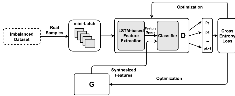
Fig. 2. The overall architecture of our model.
