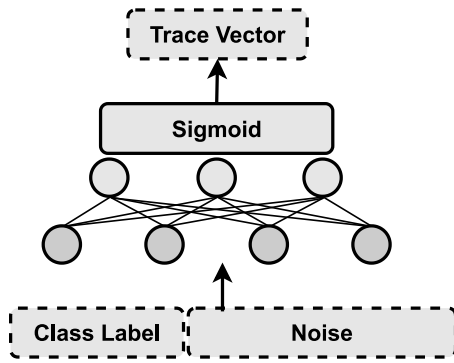
Fig. 4. Structure of class-conditioned generator network.
