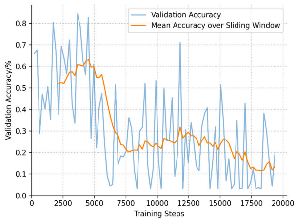
Fig. 8. Updating the running average using synthesized feature representations leads to model collapse.
