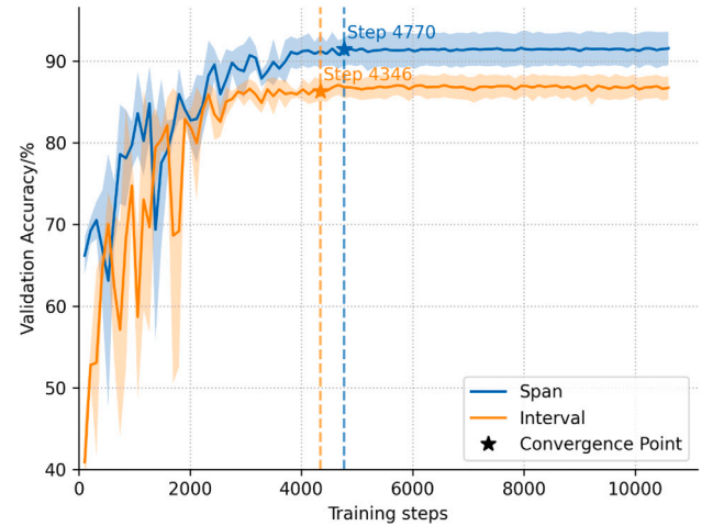
Fig. 9. Impact of trace segmentation methods on performance.
