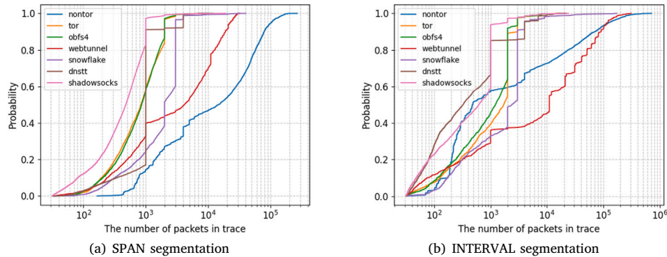
Fig. 6. CDFs of trace lengths under the two segmentation methods.
