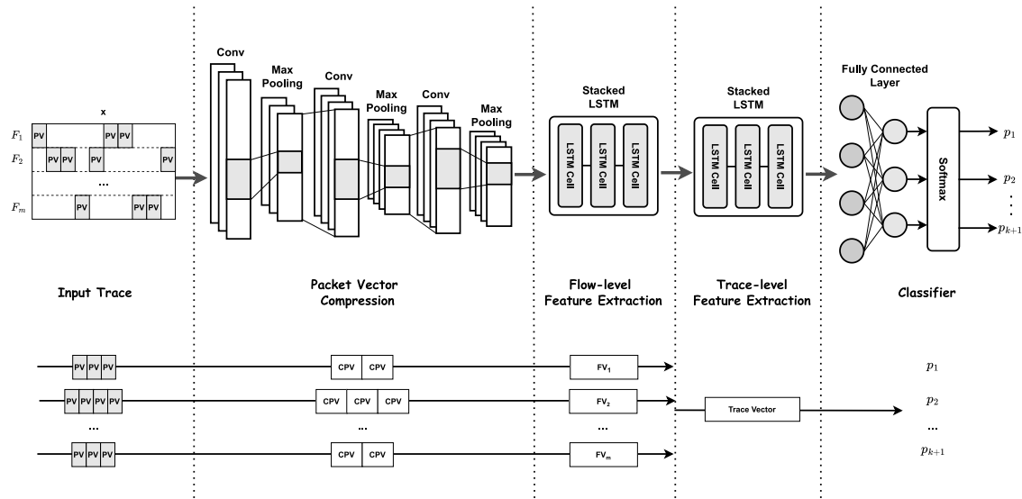
Fig. 3. Structure of discriminator network and transformation of input.
