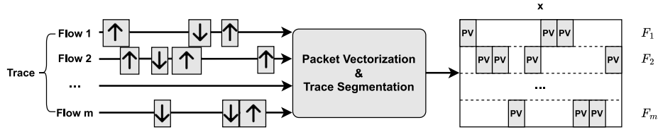
Fig. 1. An example of the hierarchical structure of a trace.
