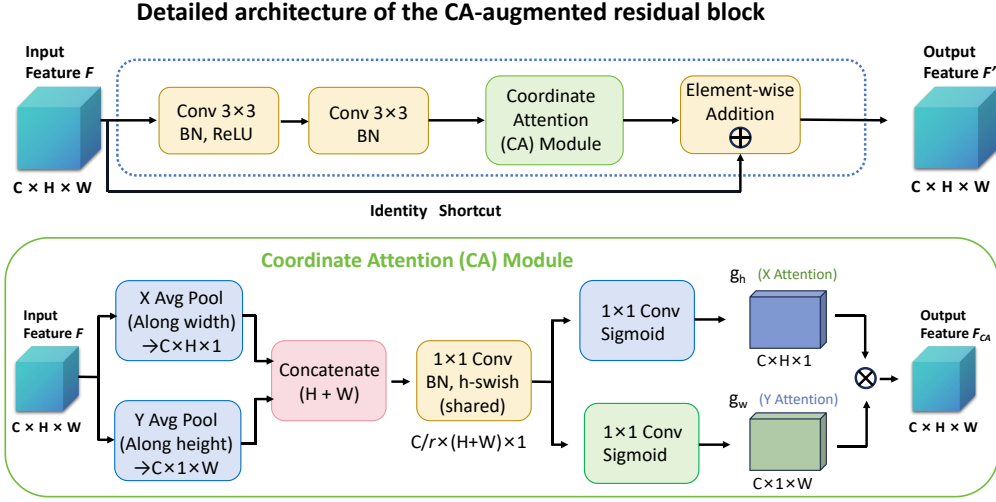
Figure 3: Detailed architecture of the CA-augmented residual block.
