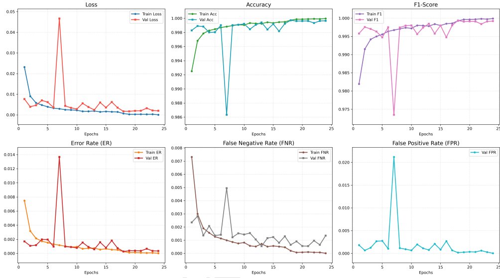
Figure 4: Training and validation dynamics of MSTE-CAN. The subplots illustrate the convergence of Loss, Accuracy, F1-Score, Error Rate (ER), FNR, and FPR over 24 epochs.
