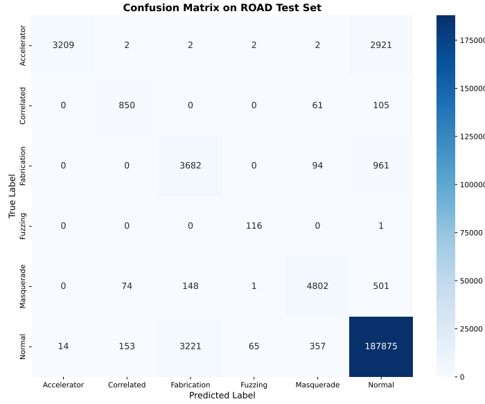
Figure 6: Confusion matrix of MSTE-CAN on the ROAD test set. The matrix reveals that Accelerator attacks are predominantly misclassified as Normal traffic, consistent with their physical-domain nature, while Fabrication attacks exhibit dispersion across multiple classes due to internal signal heterogeneity.
