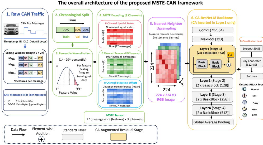
Figure 1: The overall architecture of the proposed MSTE-CAN framework. The pipeline consists of seven stages: (1) Raw CAN traffic acquisition via sliding window; (2) Chronological data partitioning; (3) Percentile normalization; (4) MSTE encoding into three-channel R/G/B tensors capturing spatial state, temporal difference, and statistical offset; (5) Nearest-neighbor upsampling to preserve field boundaries; (6) Feature extraction via CA-ResNet-18 with Coordinate Attention; and (7) Classification head outputting predictions across five attack/normal classes.
