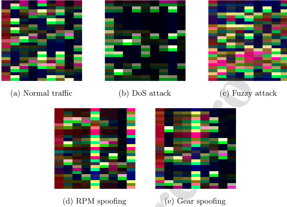
Figure 2: Visual signatures of CAN traffic under MSTE encoding. Normal traffic exhibits stable, repetitive color blocks; DoS attacks manifest as intense horizontal stripes due to high-frequency injections; Fuzzy attacks present chaotic salt-and-pepper noise patterns; Spoofing attacks show localized color shifts in specific feature columns while maintaining an overall stable structure.
