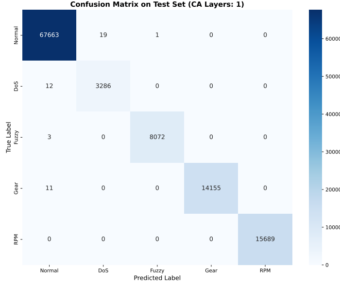
Figure 5: Confusion matrix of MSTE-CAN on the independent test set.
