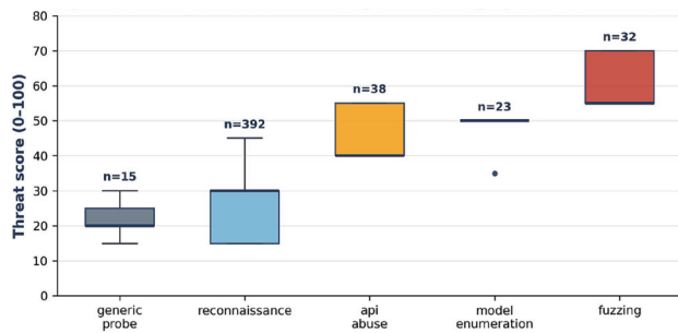
Fig. 8 Threat-score distribution by attack category in the 500-event live window (boxplots). The classifier produces a clear monotonic ranking by category
