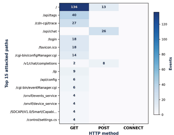
Fig. 11 HTTP method × path attack-surface heatmap (top 15 paths in the 500-event live window). POST requests concentrate on LLM-API-specific endpoints
