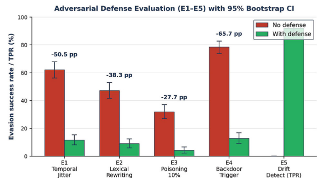
Fig. 5 Adversarial defense evaluation. Evasion success rates (E1–E4) and drift detection true-positive rate (E5) without and with the triangulation defense, with 95% bootstrap confidence intervals
