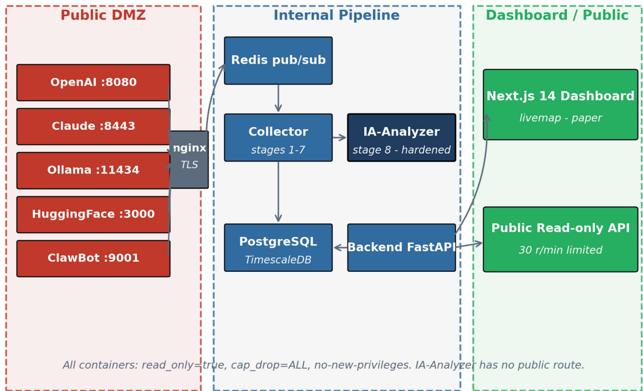
Fig. 2 HIVE-AI three-zone Docker architecture. The DMZ (left) hosts the five LLM API facades and the nginx TLS proxy. The internal pipeline zone (center) hosts Redis, the eight-stage collector, the
