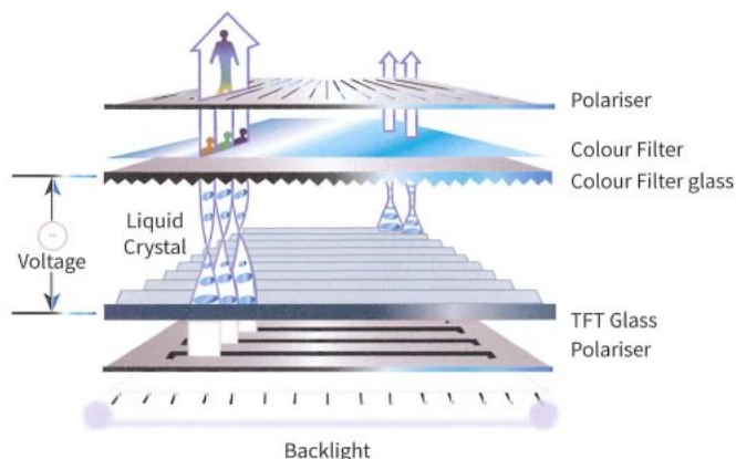
Figure 3.04 The components of a liquid-crystal display screen
