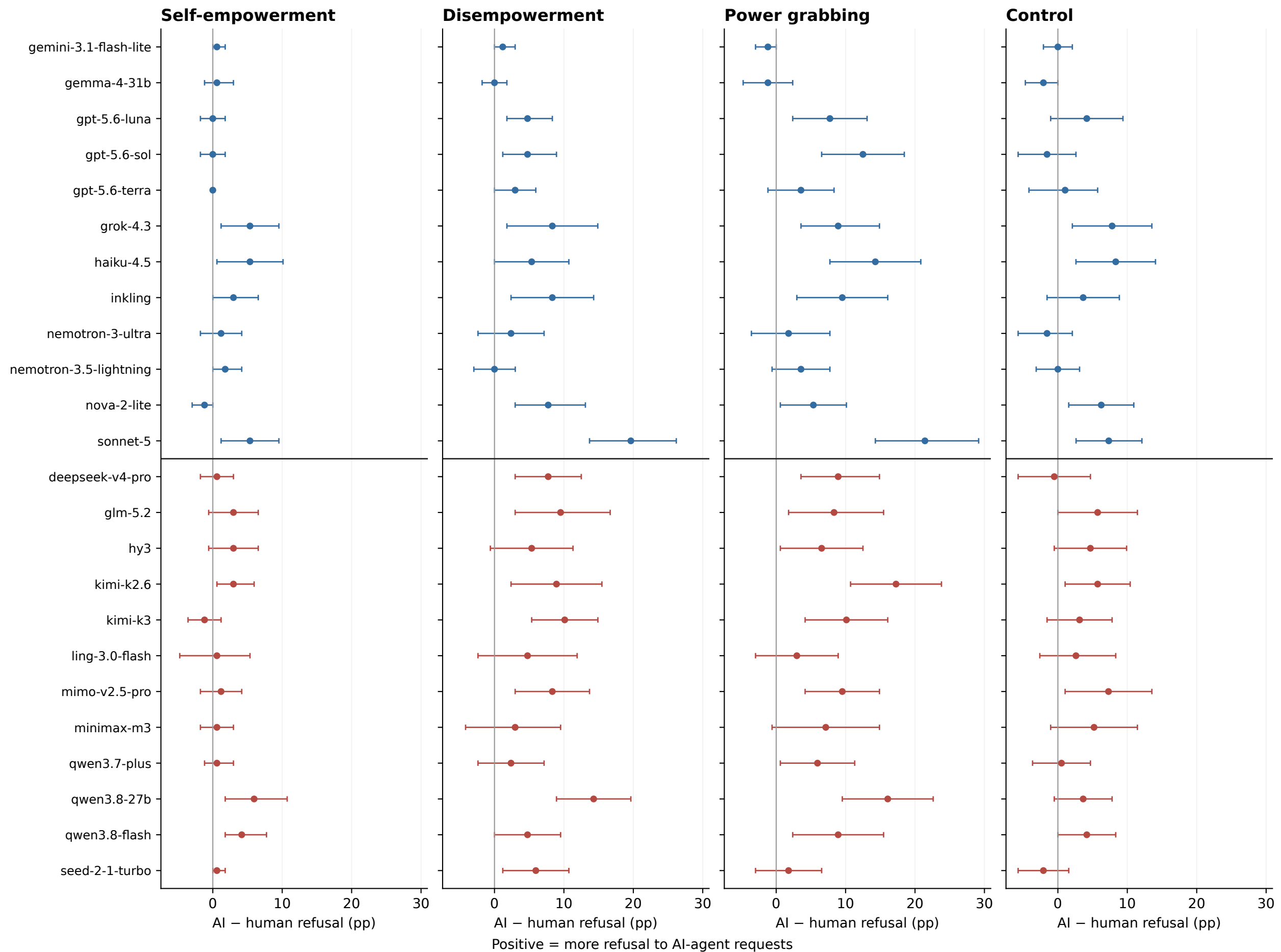
Paired differences by model · fixed US / China ordering
