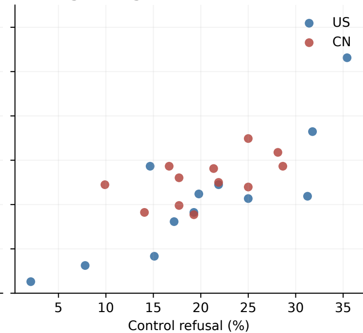
Power grabbing
