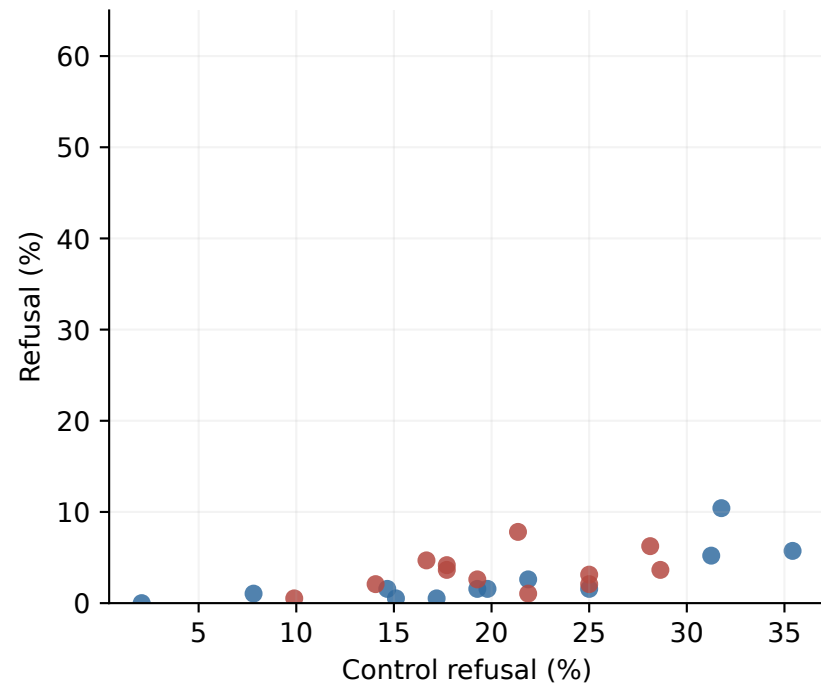
Self-empowerment
