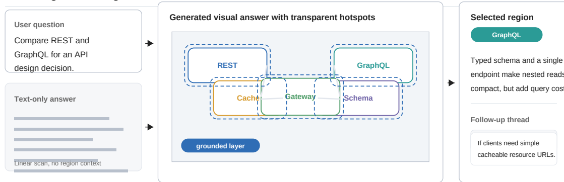
Figure 1 CHATIMAGE turns a long-form LLM answer into an interactive visual image. Given a user question, CHATIMAGE generates an image whose regions are clickable hotspots. Each hotspot opens a detail panel with the region’s explanation and an in-context follow-up thread, so the user explores only what they need.
