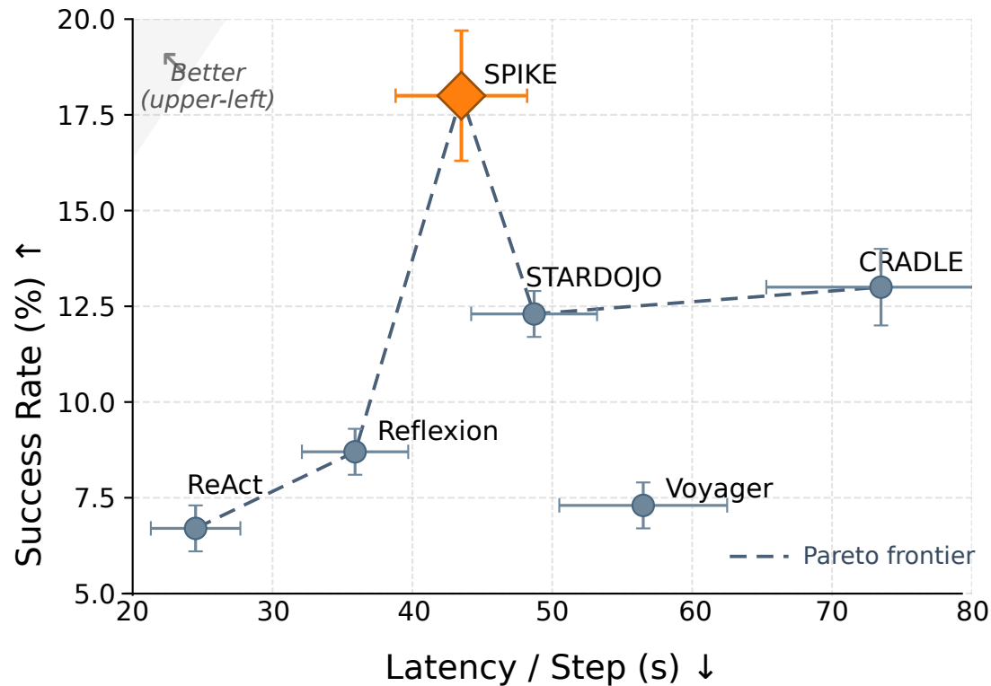
Success vs. Latency / Step
