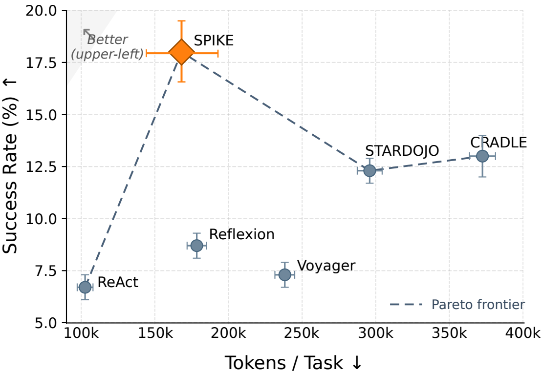
Success vs. Tokens / Task
