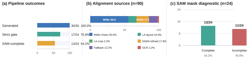
Figure 4 Experimental metric summary. Core completion and alignment results, diagnostic alignment-source distribution, and the SAM mask-completeness check; SAM-complete requires masks without obvious holes or empty cavities.
