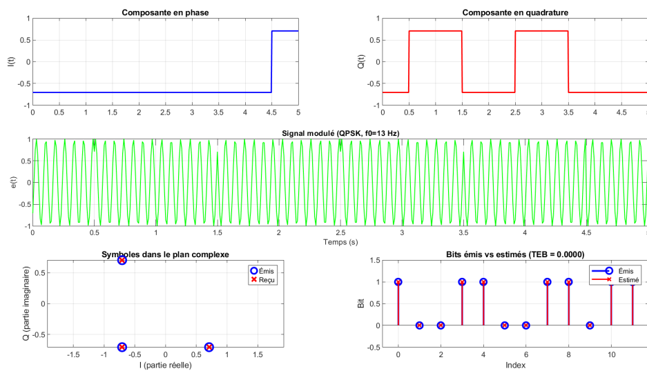
FIGURE 7 – Modulation : composantes I/Q, signal modulé, plan complexe
